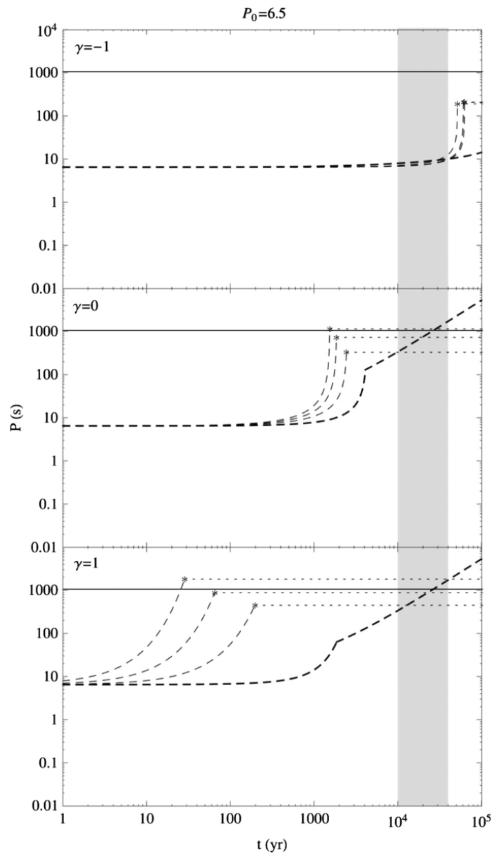
Figure 4. from Could SXP 1062 be an Accreting Magnetar? Fu & Li 2012 ApJ 757 171 doi:10.1088/0004-637X/757/2/171 https://dx.doi.org/10.1088/0004-637X/757/2/171 © 2012. The American Astronomical Society. All rights reserved.
