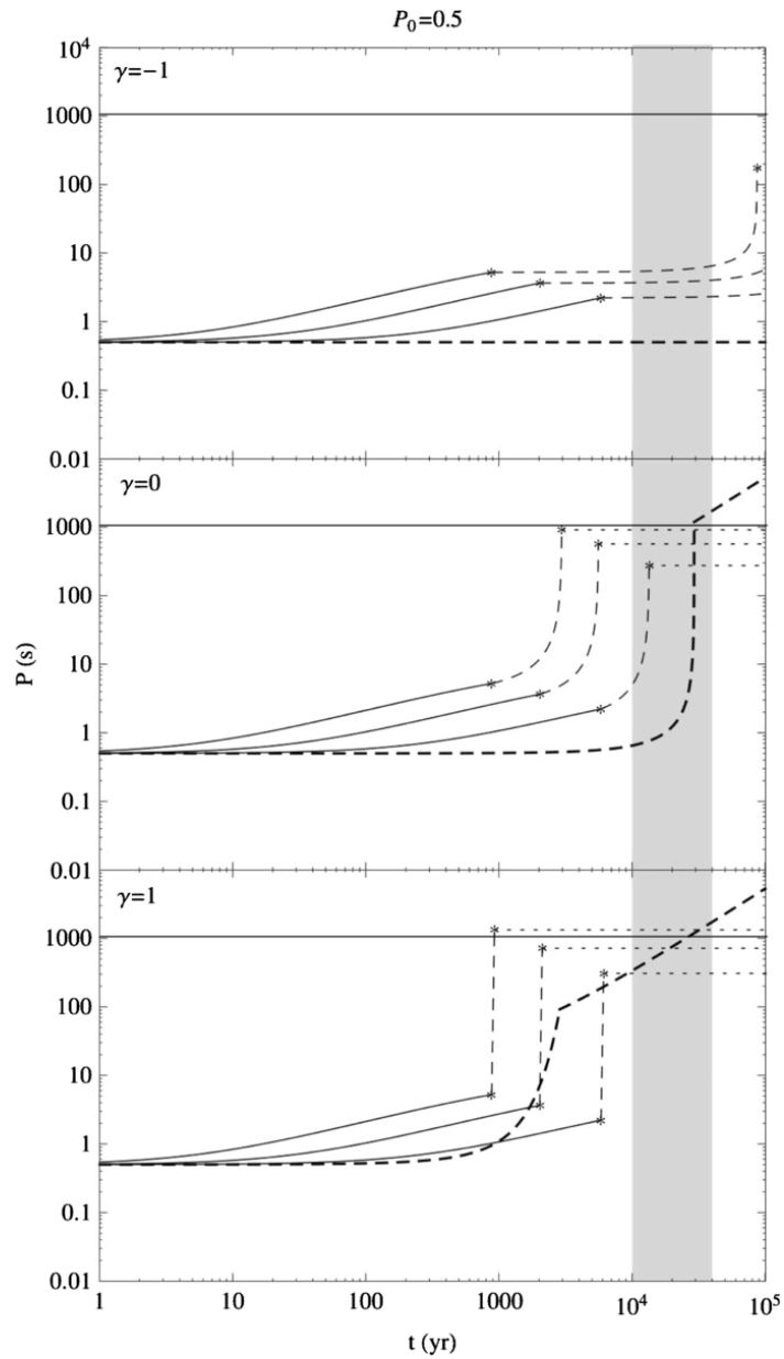
Figure 3. from Could SXP 1062 be an Accreting Magnetar? Fu & Li 2012 ApJ 757 171 doi:10.1088/0004-637X/757/2/171 https://dx.doi.org/10.1088/0004-637X/757/2/171 © 2012. The American Astronomical Society. All rights reserved.
