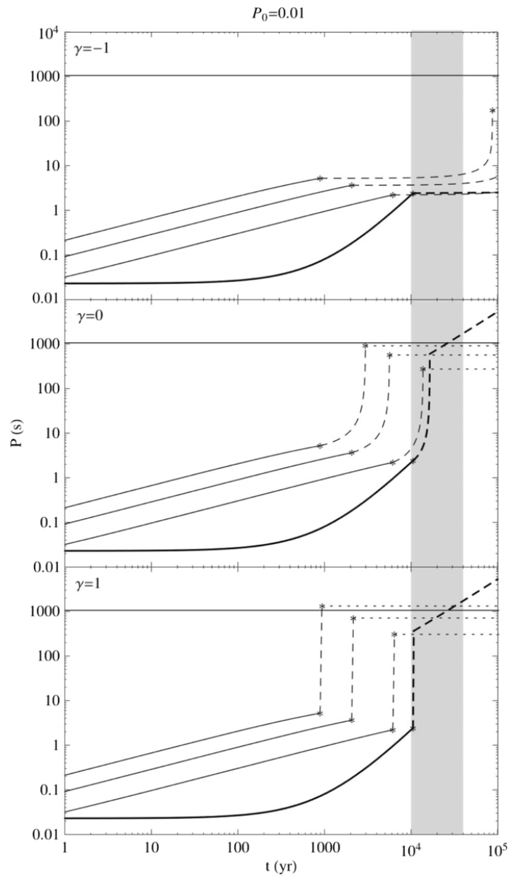
Figure 2. from Could SXP 1062 be an Accreting Magnetar? Fu & Li 2012 ApJ 757 171 doi:10.1088/0004-637X/757/2/171 https://dx.doi.org/10.1088/0004-637X/757/2/171 © 2012. The American Astronomical Society. All rights reserved.
