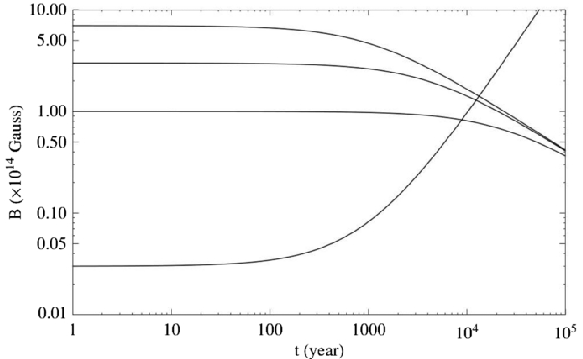
Figure 1. from Could SXP 1062 be an Accreting Magnetar? Fu & Li 2012 ApJ 757 171 doi:10.1088/0004-637X/757/2/171 https://dx.doi.org/10.1088/0004-637X/757/2/171 © 2012. The American Astronomical Society. All rights reserved.
