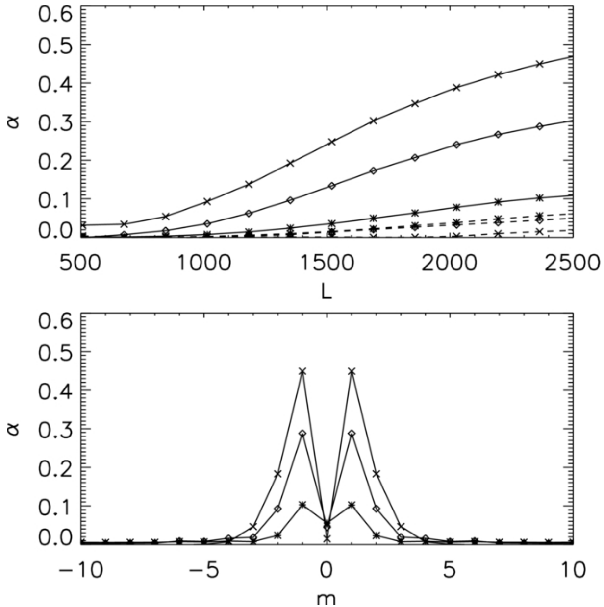
Figure 8. from Scattering of the f-mode by Small Magnetic Flux Elements from Observations and Numerical Simulations Felipe et al. 2012 ApJ 757 148 doi:10.1088/0004-637X/757/2/148 https://dx.doi.org/10.1088/0004-637X/757/2/148
