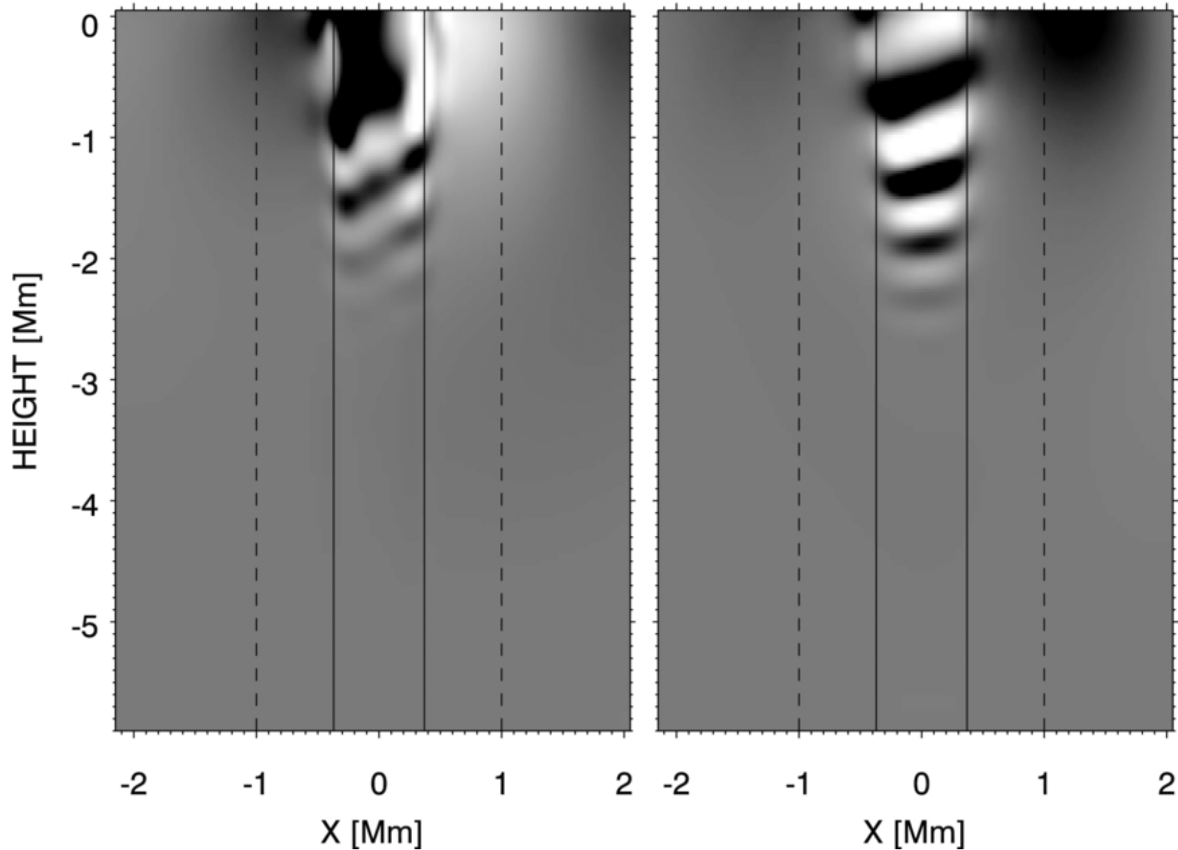
Figure 4. from Scattering of the f-mode by Small Magnetic Flux Elements from Observations and Numerical Simulations Felipe et al. 2012 ApJ 757 148 doi:10.1088/0004-637X/757/2/148 https://dx.doi.org/10.1088/0004-637X/757/2/148 © 2012. The American Astronomical Society. All rights reserved.
