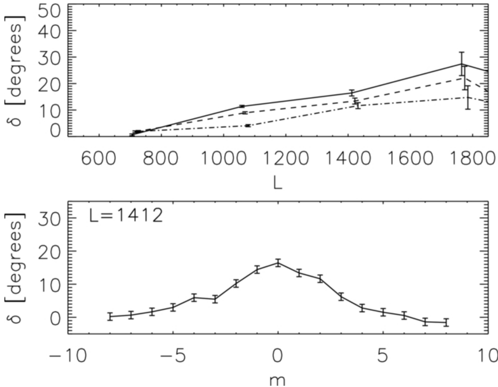
Figure 2. from Scattering of the f-mode by Small Magnetic Flux Elements from Observations and Numerical Simulations Felipe et al. 2012 ApJ 757 148 doi:10.1088/0004-637X/757/2/148 https://dx.doi.org/10.1088/0004-637X/757/2/148 © 2012. The American Astronomical Society. All rights reserved.
