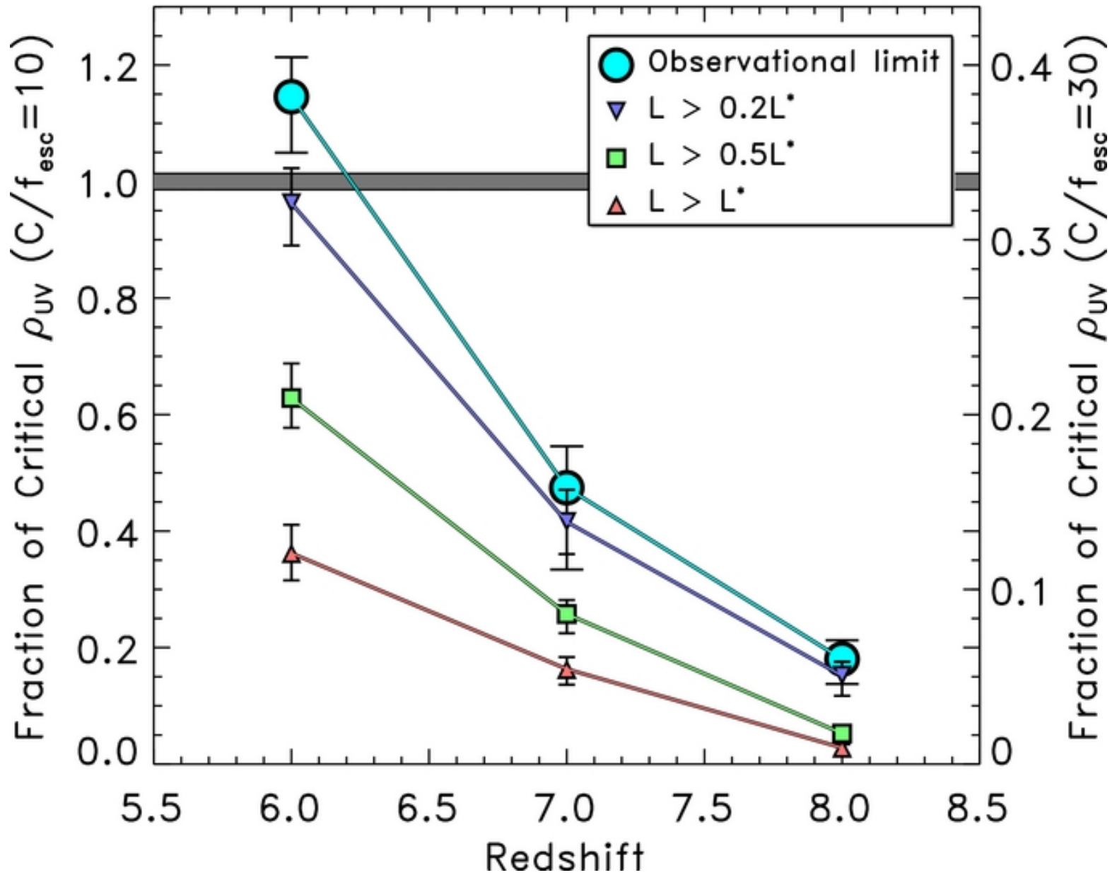
Figure 4. from CANDELS: The Contribution of the Observed Galaxy Population to Cosmic Reionization Finkelstein et al. 2012 ApJ 758 93 doi:10.1088/0004-637X/758/2/93 https://dx.doi.org/10.1088/0004-637X/758/2/93 © 2012. The American Astronomical Society. All rights reserved.
