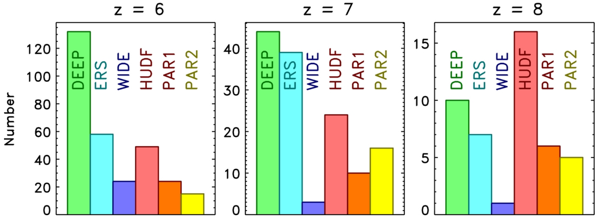
Figure 1. from CANDELS: The Contribution of the Observed Galaxy Population to Cosmic Reionization Finkelstein et al. 2012 ApJ 758 93 doi:10.1088/0004-637X/758/2/93 https://dx.doi.org/10.1088/0004-637X/758/2/93 © 2012. The American Astronomical Society. All rights reserved.
