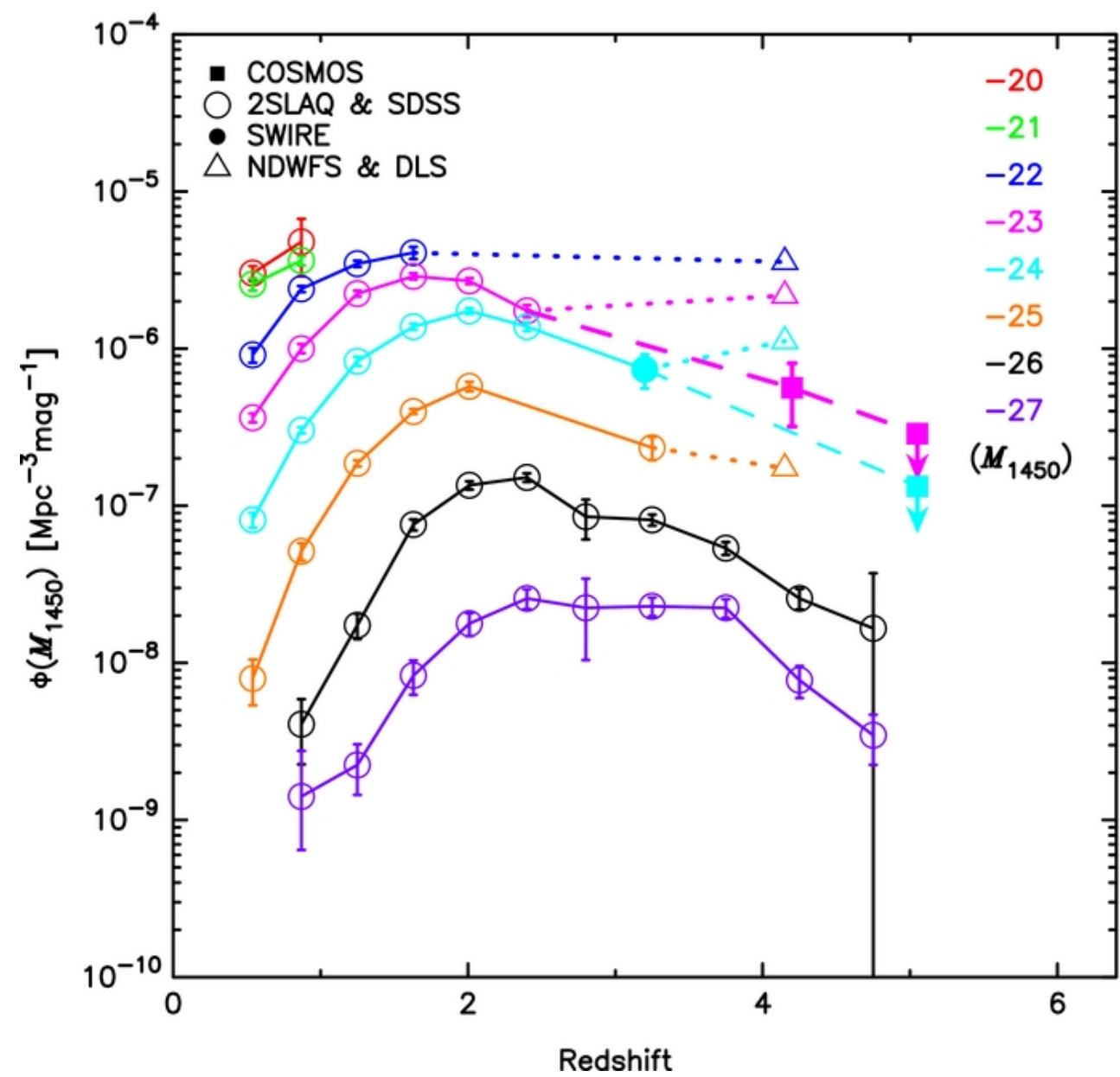
Figure 9. from Constraints on the Faint End of the Quasar Luminosity Function at z \sim 5 in the COSMOS Field Ikeda et al. 2012 ApJ 756 160 doi:10.1088/0004-637X/756/2/160 https://dx.doi.org/10.1088/0004-637X/756/2/160 © 2012. The American Astronomical Society. All rights reserved.
