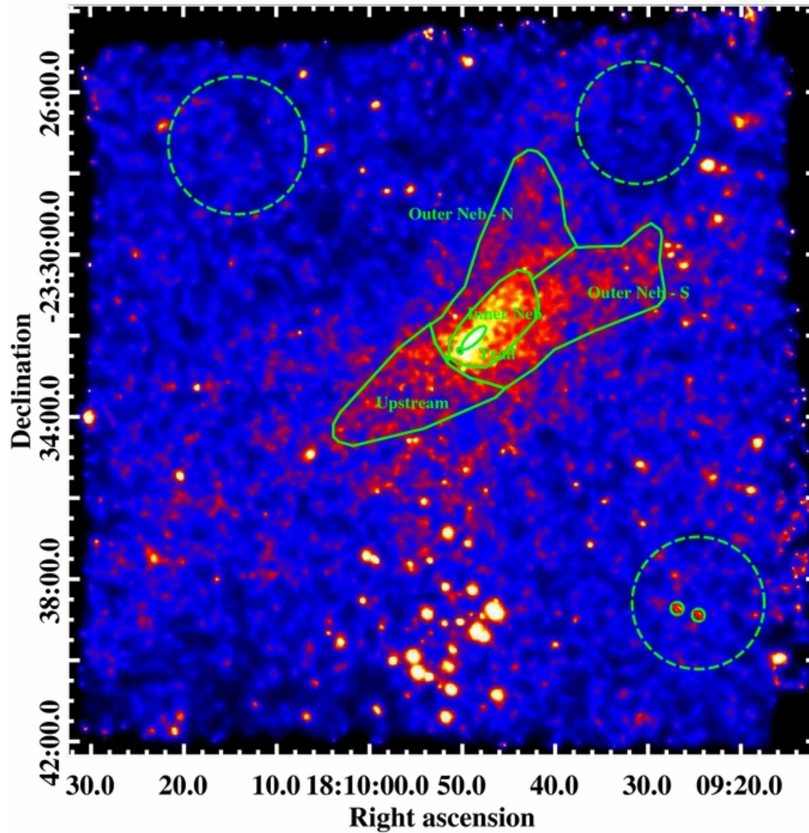
Figure 5. from A Chandra Proper Motion for PSR J1809–2332 Van Etten, Romani, & Ng 2012 ApJ 755 151 doi:10.1088/0004-637X/755/2/151 https://dx.doi.org/10.1088/0004-637X/755/2/151 © 2012. The American Astronomical Society. All rights reserved.
