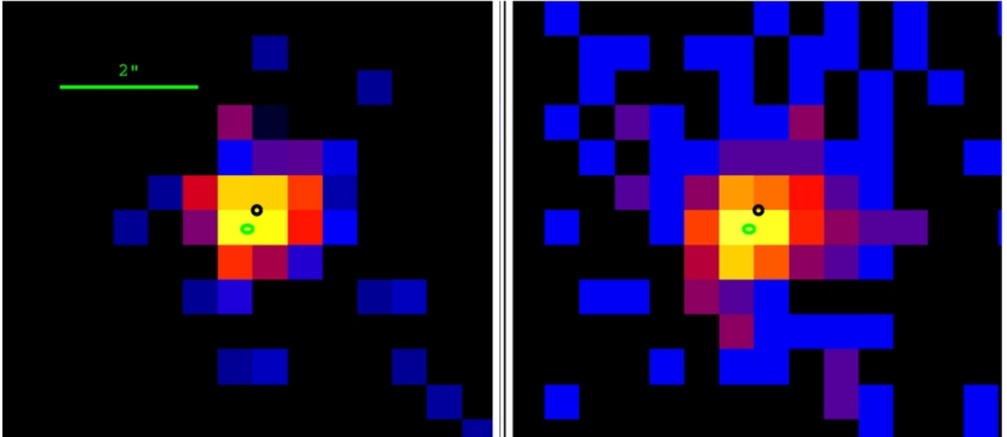
Figure 4. from A Chandra Proper Motion for PSR J1809–2332 Van Etten, Romani, & Ng 2012 ApJ 755 151 doi:10.1088/0004-637X/755/2/151 https://dx.doi.org/10.1088/0004-637X/755/2/151 © 2012. The American Astronomical Society. All rights reserved.
