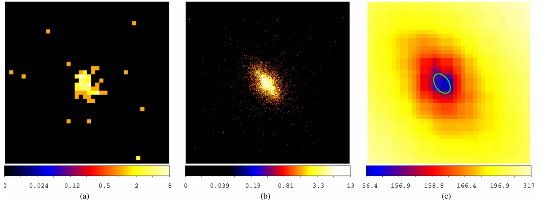
Figure 2. from A Chandra Proper Motion for PSR J1809–2332 Van Etten, Romani, & Ng 2012 ApJ 755 151 doi:10.1088/0004-637X/755/2/151 https://dx.doi.org/10.1088/0004-637X/755/2/151 © 2012. The American Astronomical Society. All rights reserved.
