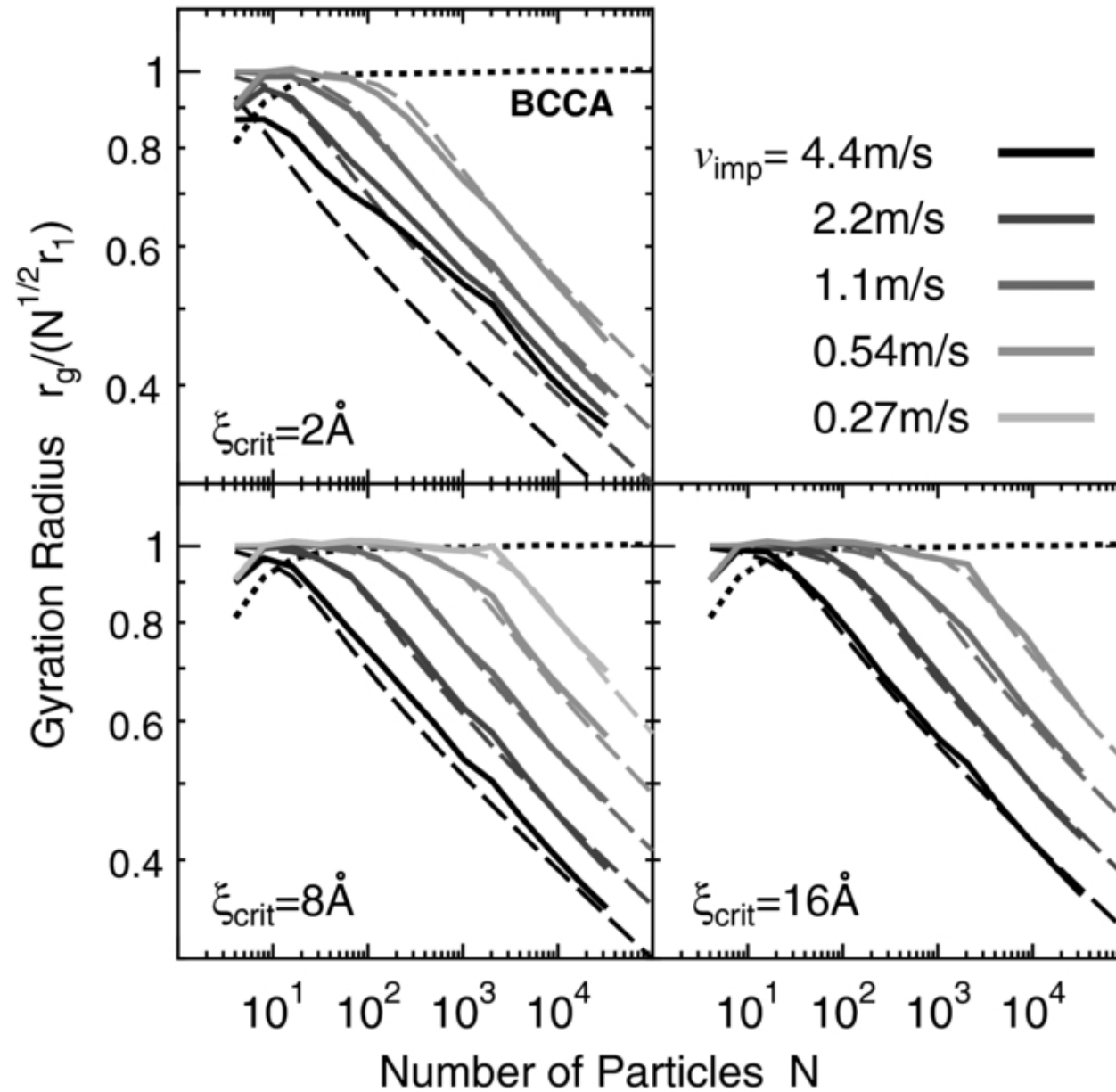
Figure 9. from Geometric Cross Sections of Dust Aggregates and a Compression Model for Aggregate Collisions Suyama et al. 2012 ApJ 753 115 doi:10.1088/0004-637X/753/2/115 https://dx.doi.org/10.1088/0004-637X/753/2/115 © 2012. The American Astronomical Society. All rights reserved.
