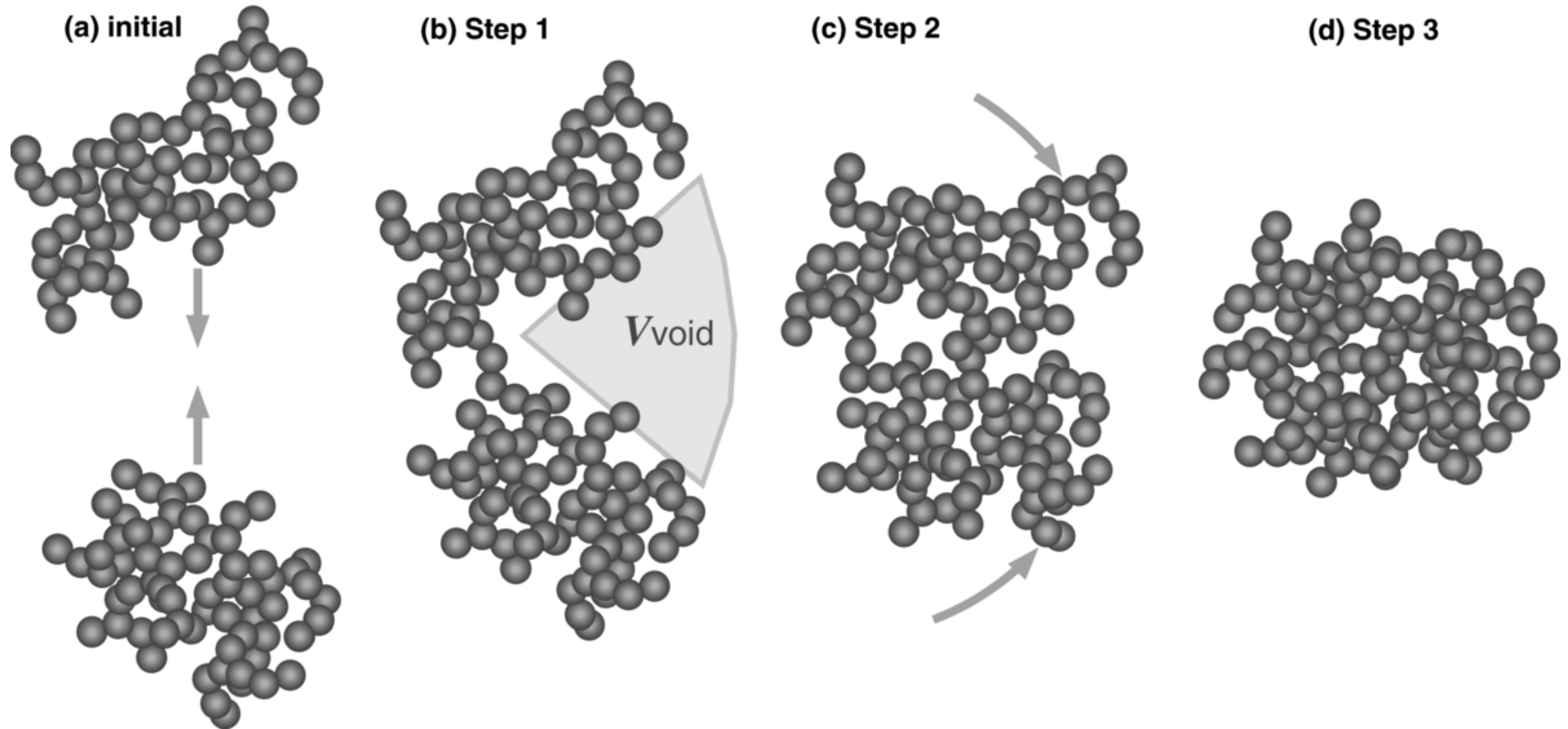
Figure 8. from Geometric Cross Sections of Dust Aggregates and a Compression Model for Aggregate Collisions Suyama et al. 2012 ApJ 753 115 doi:10.1088/0004-637X/753/2/115 https://dx.doi.org/10.1088/0004-637X/753/2/115 © 2012. The American Astronomical Society. All rights reserved.
