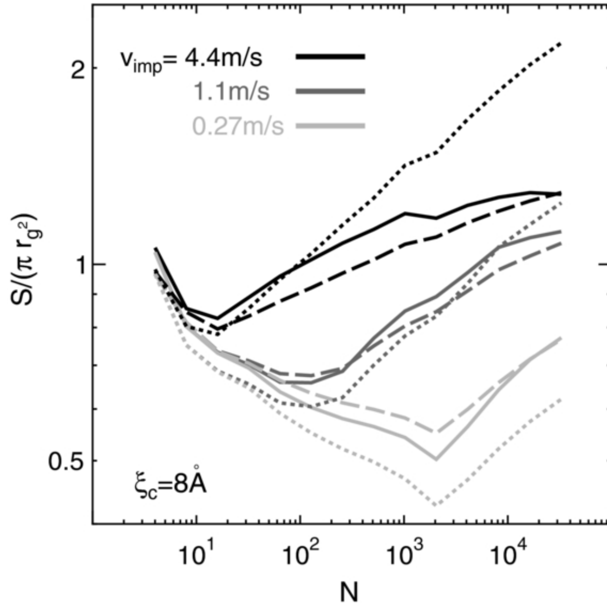
Figure 7. from Geometric Cross Sections of Dust Aggregates and a Compression Model for Aggregate Collisions Suyama et al. 2012 ApJ 753 115 doi:10.1088/0004-637X/753/2/115 https://dx.doi.org/10.1088/0004-637X/753/2/115 © 2012. The American Astronomical Society. All rights reserved.
