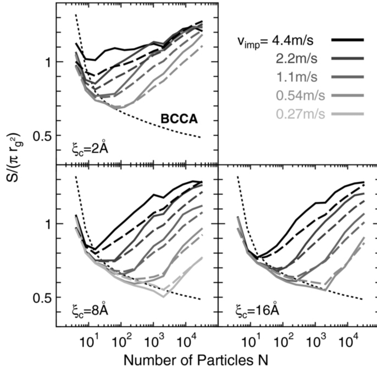
Figure 6. from Geometric Cross Sections of Dust Aggregates and a Compression Model for Aggregate Collisions Suyama et al. 2012 ApJ 753 115 doi:10.1088/0004-637X/753/2/115 https://dx.doi.org/10.1088/0004-637X/753/2/115 © 2012. The American Astronomical Society. All rights reserved.
