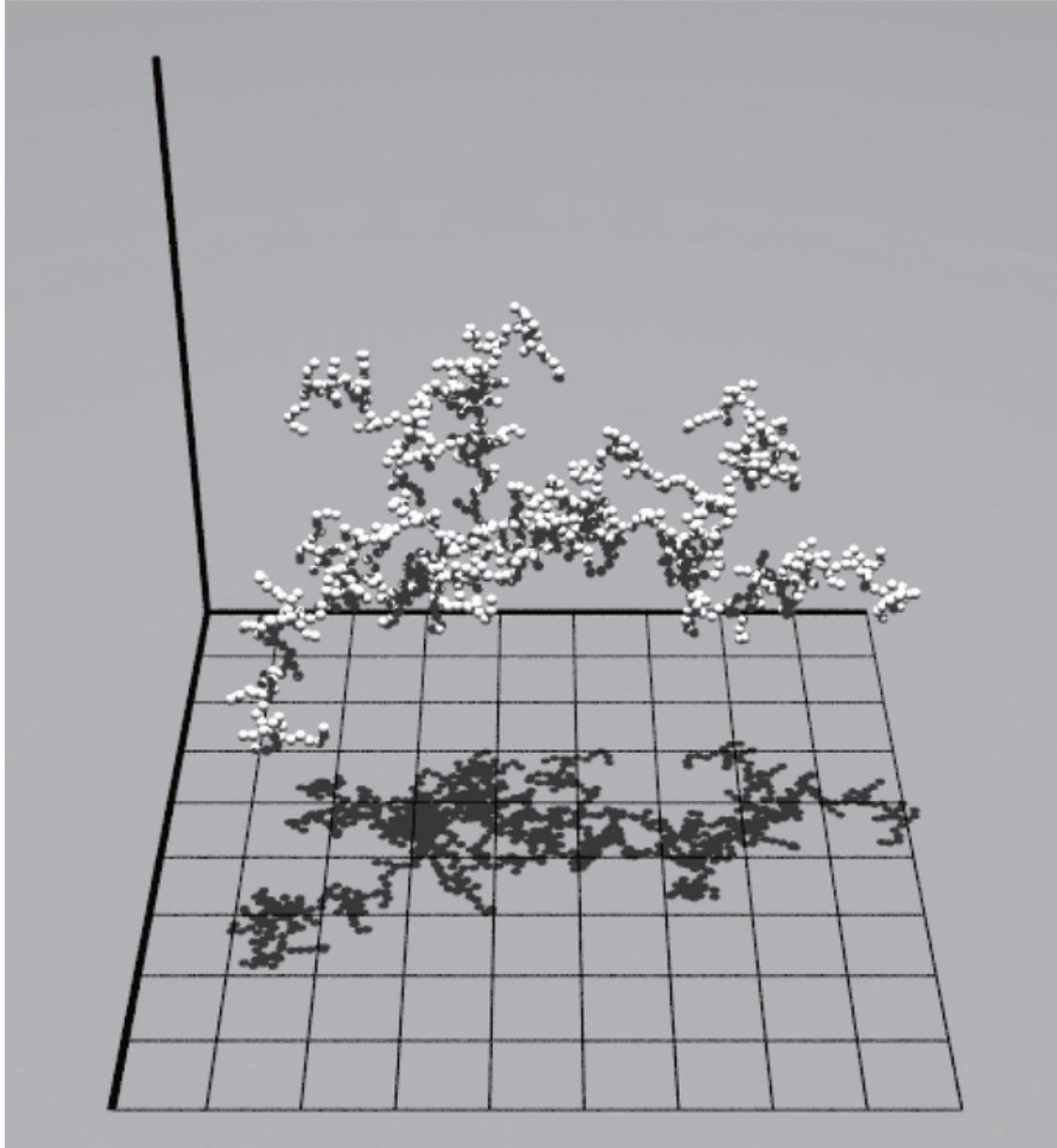
Figure 3. from Geometric Cross Sections of Dust Aggregates and a Compression Model for Aggregate Collisions Suyama et al. 2012 ApJ 753 115 doi:10.1088/0004-637X/753/2/115 https://dx.doi.org/10.1088/0004-637X/753/2/115 © 2012. The American Astronomical Society. All rights reserved.
