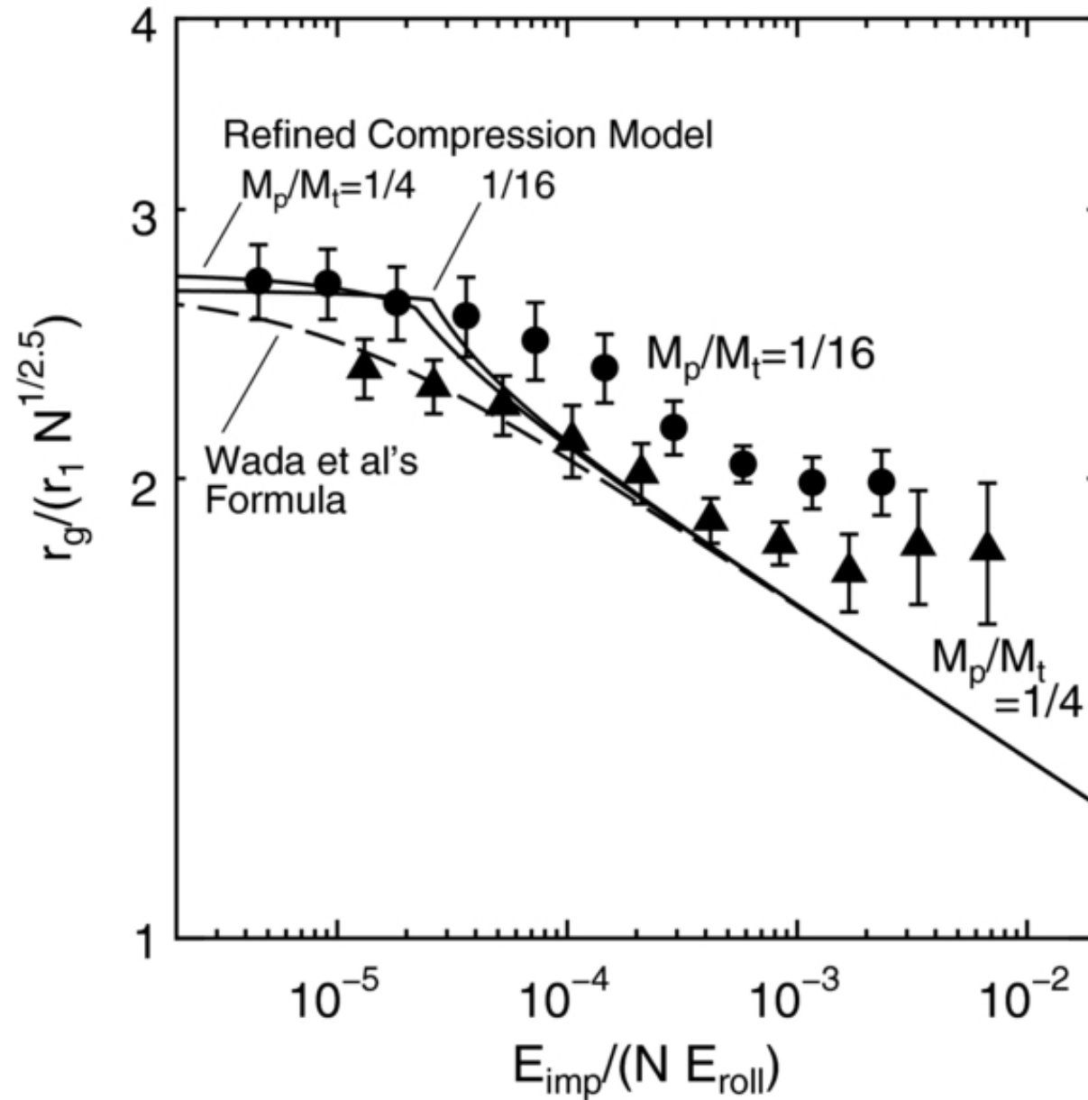
Figure 12. from Geometric Cross Sections of Dust Aggregates and a Compression Model for Aggregate Collisions Suyama et al. 2012 ApJ 753 115 doi:10.1088/0004-637X/753/2/115 https://dx.doi.org/10.1088/0004-637X/753/2/115 © 2012. The American Astronomical Society. All rights reserved.
