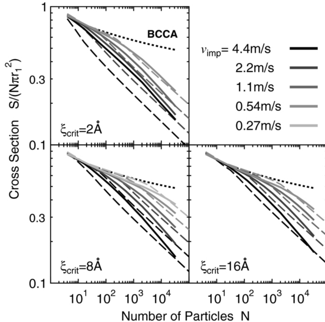
Figure 10. from Geometric Cross Sections of Dust Aggregates and a Compression Model for Aggregate Collisions Suyama et al. 2012 ApJ 753 115 doi:10.1088/0004-637X/753/2/115 https://dx.doi.org/10.1088/0004-637X/753/2/115 © 2012. The American Astronomical Society. All rights reserved.
