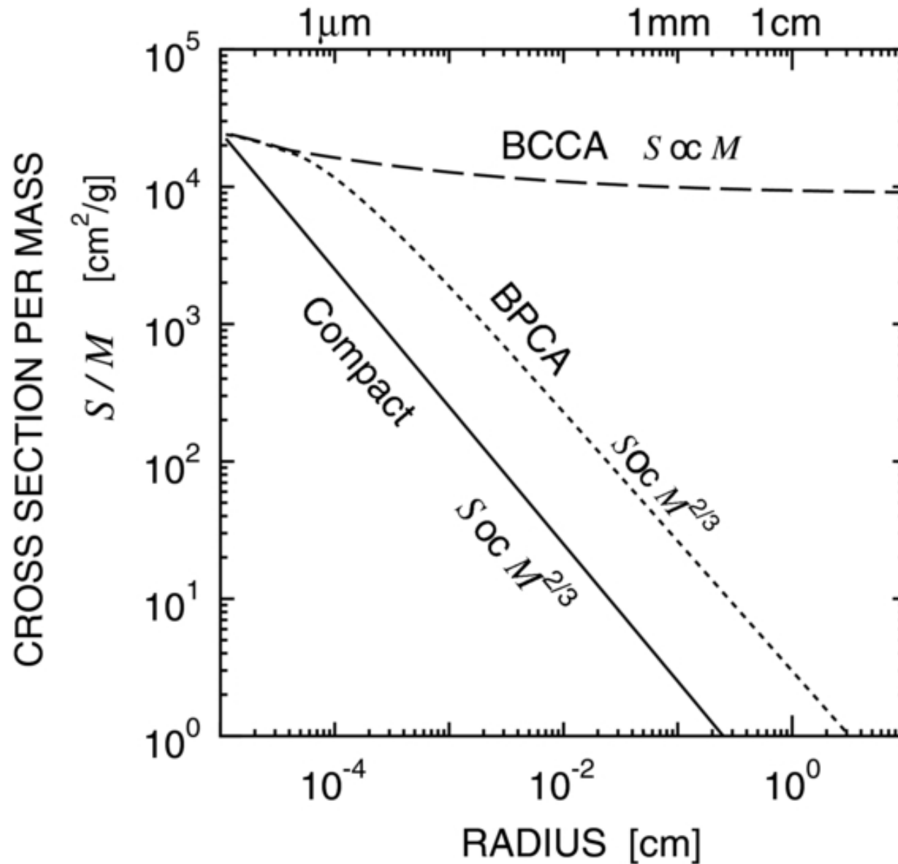
Figure 1. from Geometric Cross Sections of Dust Aggregates and a Compression Model for Aggregate Collisions Suyama et al. 2012 ApJ 753 115 doi:10.1088/0004-637X/753/2/115 https://dx.doi.org/10.1088/0004-637X/753/2/115 © 2012. The American Astronomical Society. All rights reserved.
