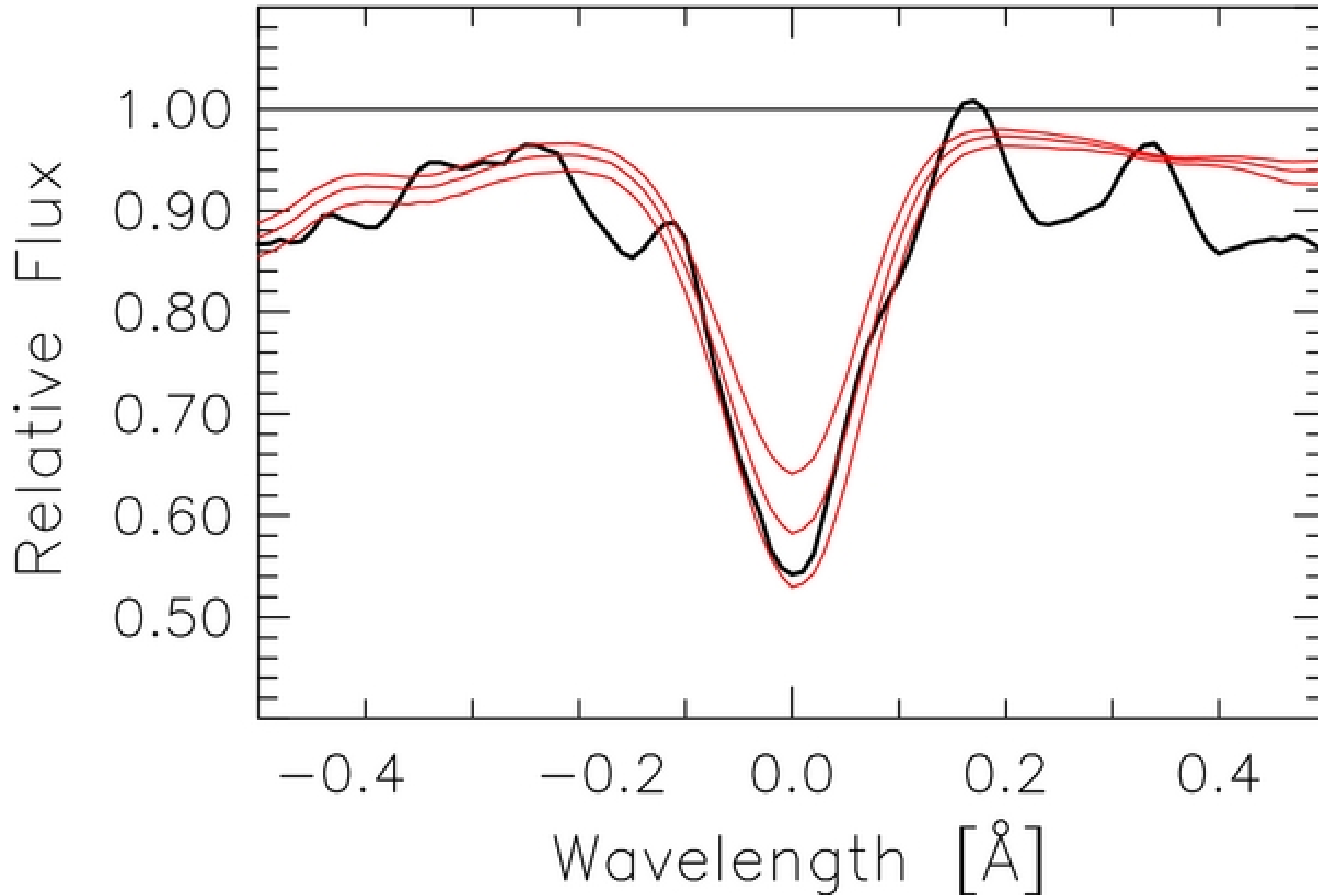
Figure 3. from The Oxygen Abundance of the Ultra-metal-poor Star HE 0557–4840 Norris et al. 2012 ApJ 753 150 doi:10.1088/0004-637X/753/2/150 https://dx.doi.org/10.1088/0004-637X/753/2/150 © 2012. The American Astronomical Society. All rights reserved.
