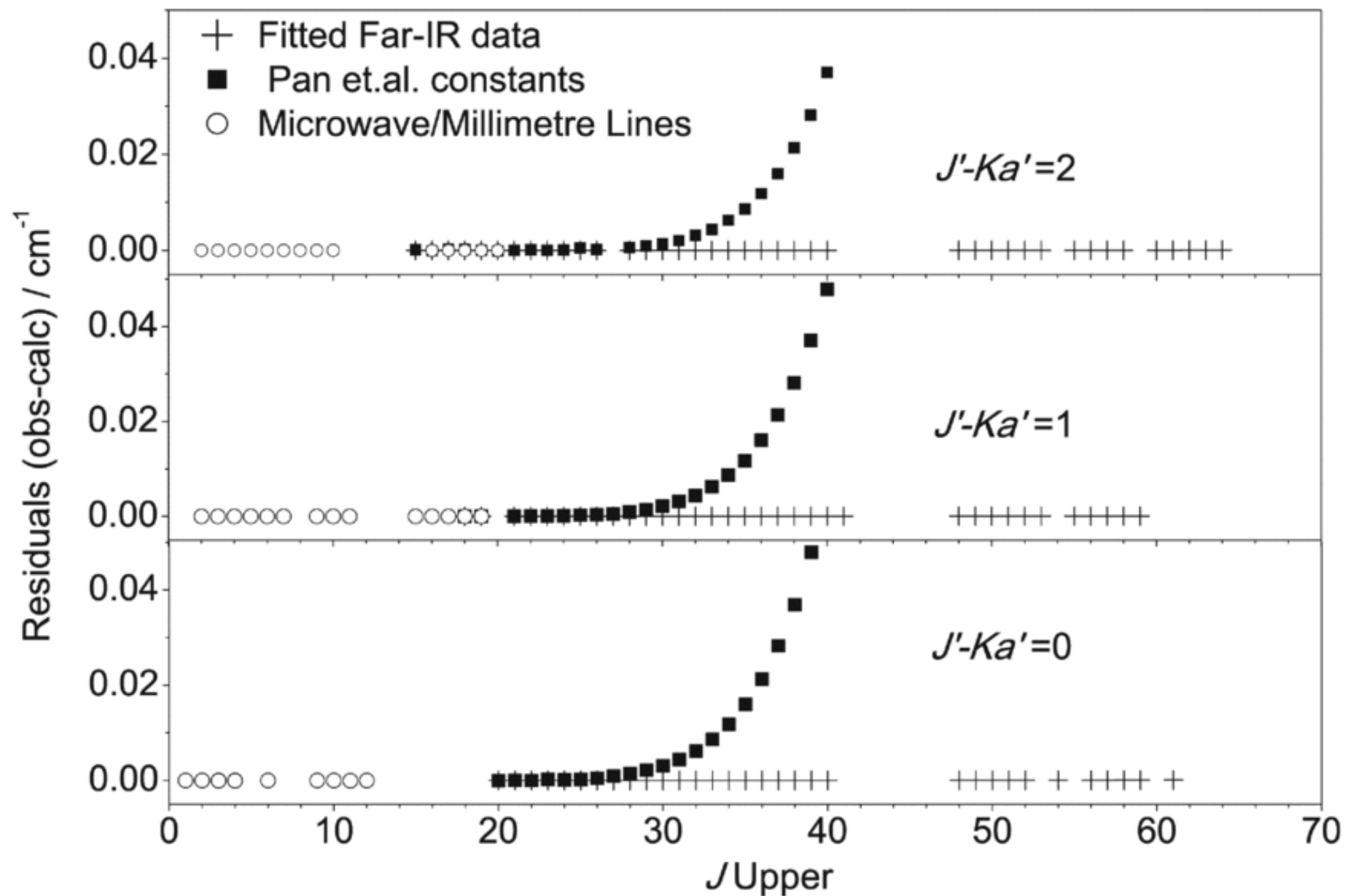
Figure 3. from The Far-infrared Rotational Spectrum of Ethylene Oxide Medcraft et al. 2012 ApJ 753 18 doi:10.1088/0004-637X/753/1/18 https://dx.doi.org/10.1088/0004-637X/753/1/18 © 2012. The American Astronomical Society. All rights reserved.
