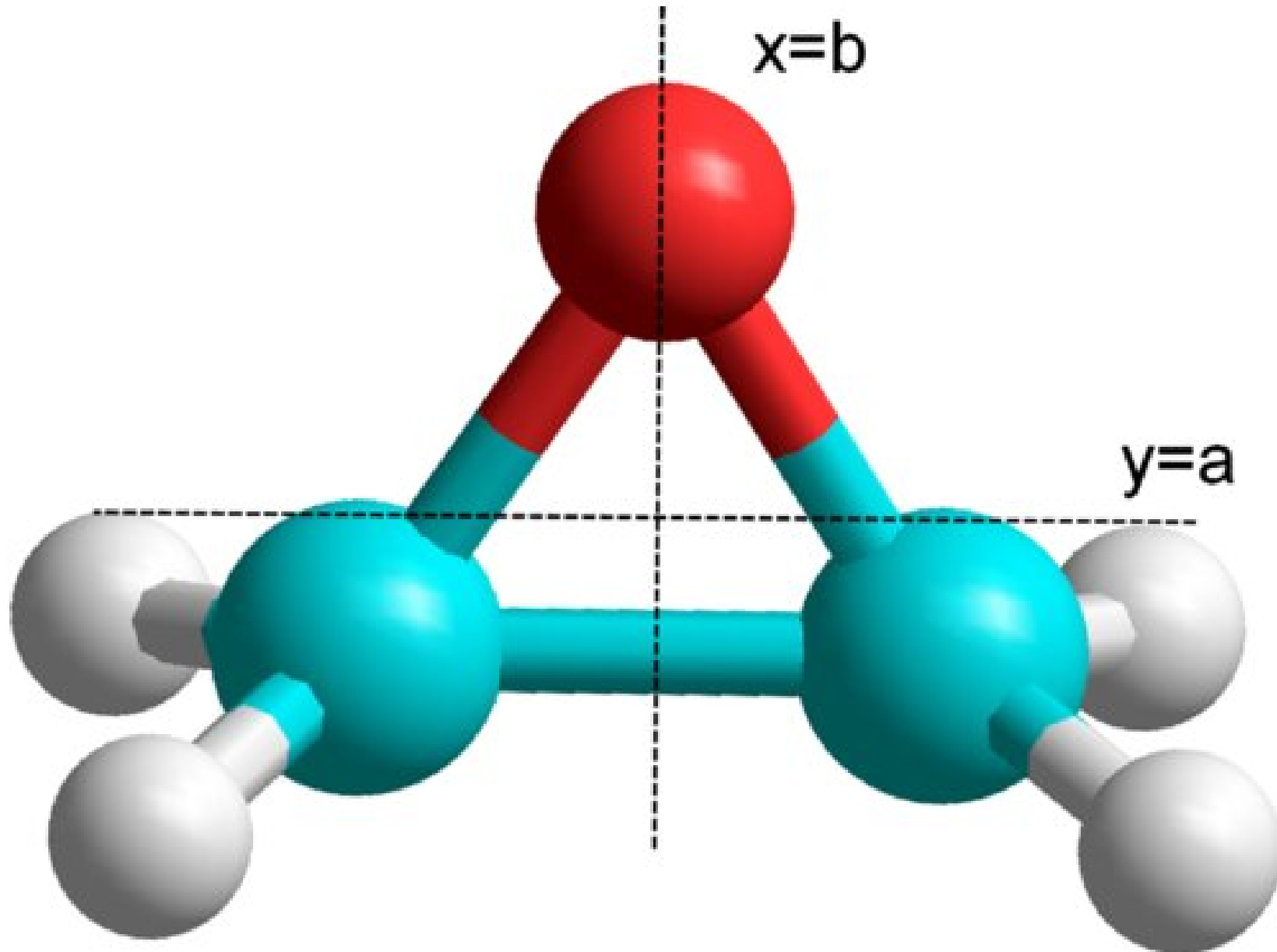
Figure 2. from The Far-infrared Rotational Spectrum of Ethylene Oxide Medcraft et al. 2012 ApJ 753 18 doi:10.1088/0004-637X/753/1/18 https://dx.doi.org/10.1088/0004-637X/753/1/18 © 2012. The American Astronomical Society. All rights reserved.
