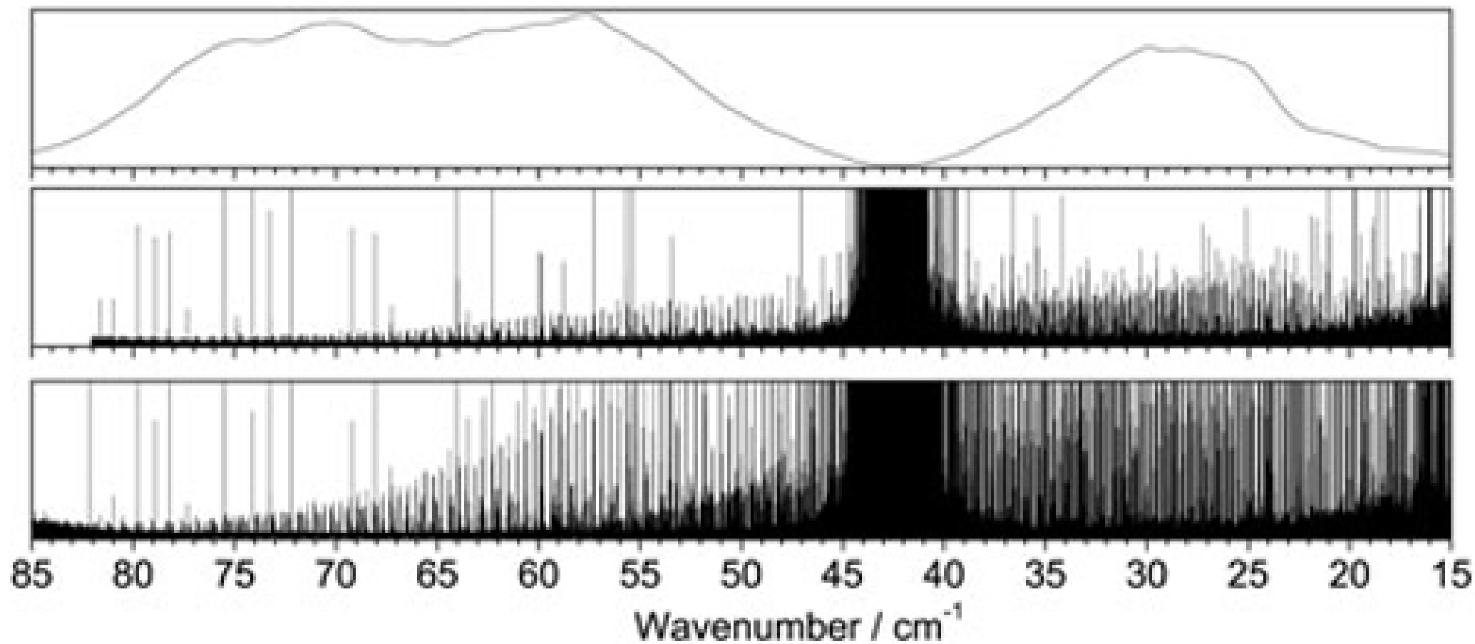
Figure 1. from The Far-infrared Rotational Spectrum of Ethylene Oxide Medcraft et al. 2012 ApJ 753 18 doi:10.1088/0004-637X/753/1/18 https://dx.doi.org/10.1088/0004-637X/753/1/18 © 2012. The American Astronomical Society. All rights reserved.
