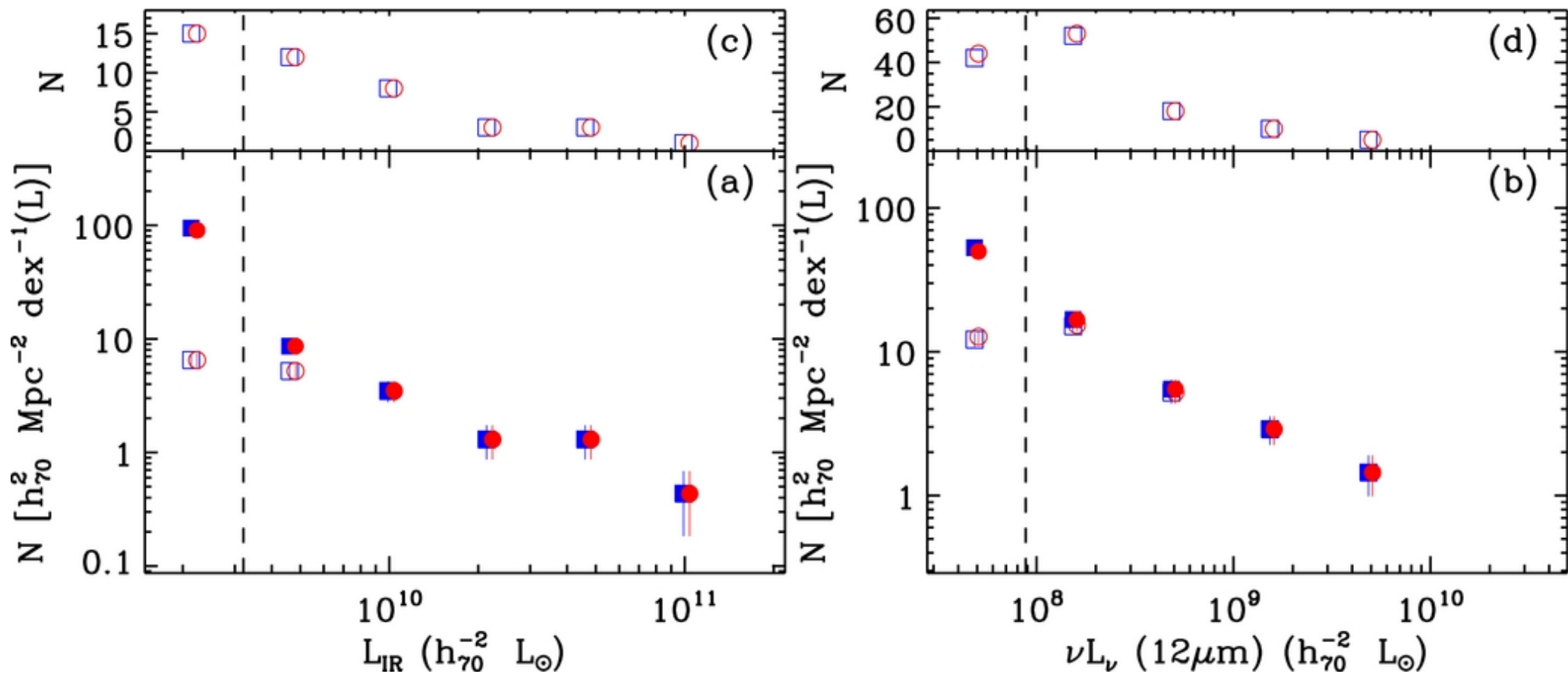
Figure 8. from A WISE View of a nearby Supercluster A2199 Hwang et al. 2012 ApJ 752 64 doi:10.1088/0004-637X/752/1/64 https://dx.doi.org/10.1088/0004-637X/752/1/64 © 2012. The American Astronomical Society. All rights reserved.
