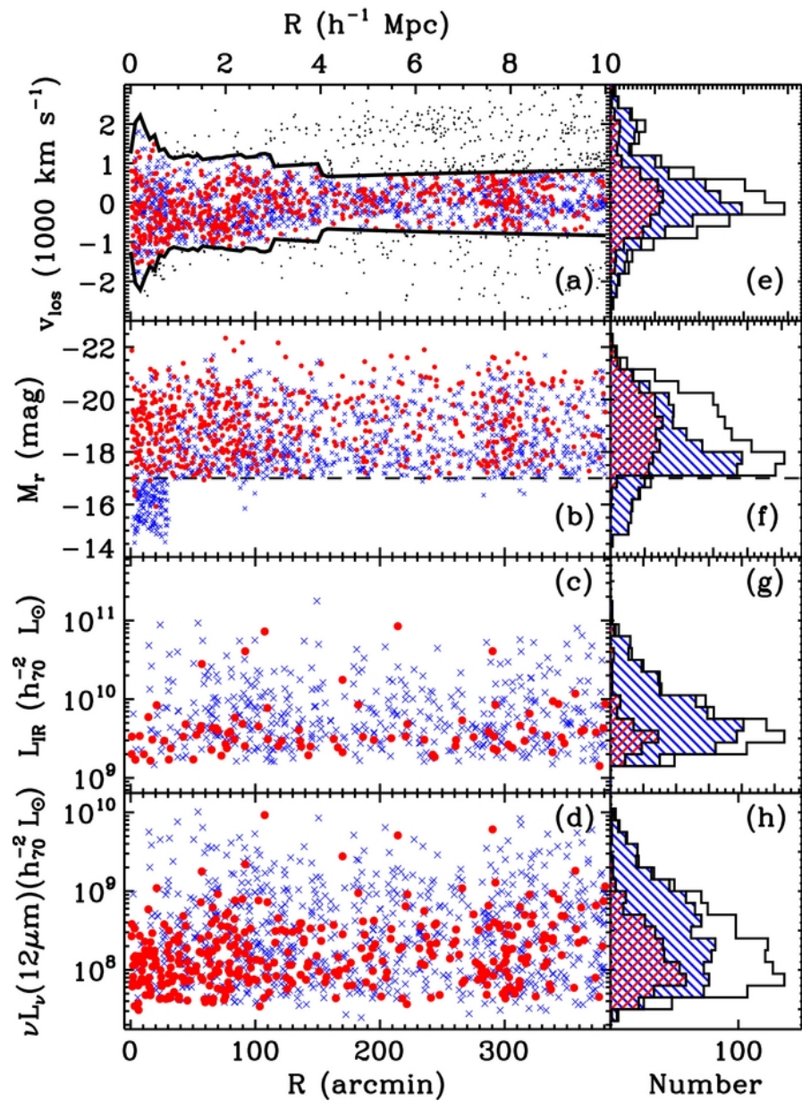
Figure 3. from A WISE View of a nearby Supercluster A2199 Hwang et al. 2012 ApJ 752 64 doi:10.1088/0004-637X/752/1/64 https://dx.doi.org/10.1088/0004-637X/752/1/64 © 2012. The American Astronomical Society. All rights reserved.
