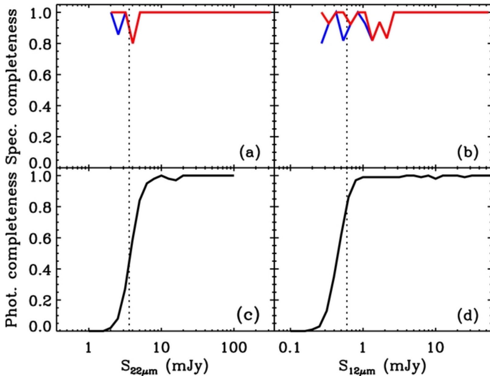
Figure 2. from A WISE View of a nearby Supercluster A2199 Hwang et al. 2012 ApJ 752 64 doi:10.1088/0004-637X/752/1/64 https://dx.doi.org/10.1088/0004-637X/752/1/64 © 2012. The American Astronomical Society. All rights reserved.
