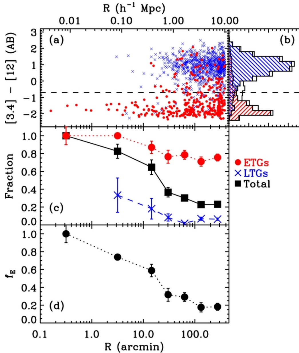
Figure 14. from A WISE View of a nearby Supercluster A2199 Hwang et al. 2012 ApJ 752 64 doi:10.1088/0004-637X/752/1/64 https://dx.doi.org/10.1088/0004-637X/752/1/64 © 2012. The American Astronomical Society. All rights reserved.
