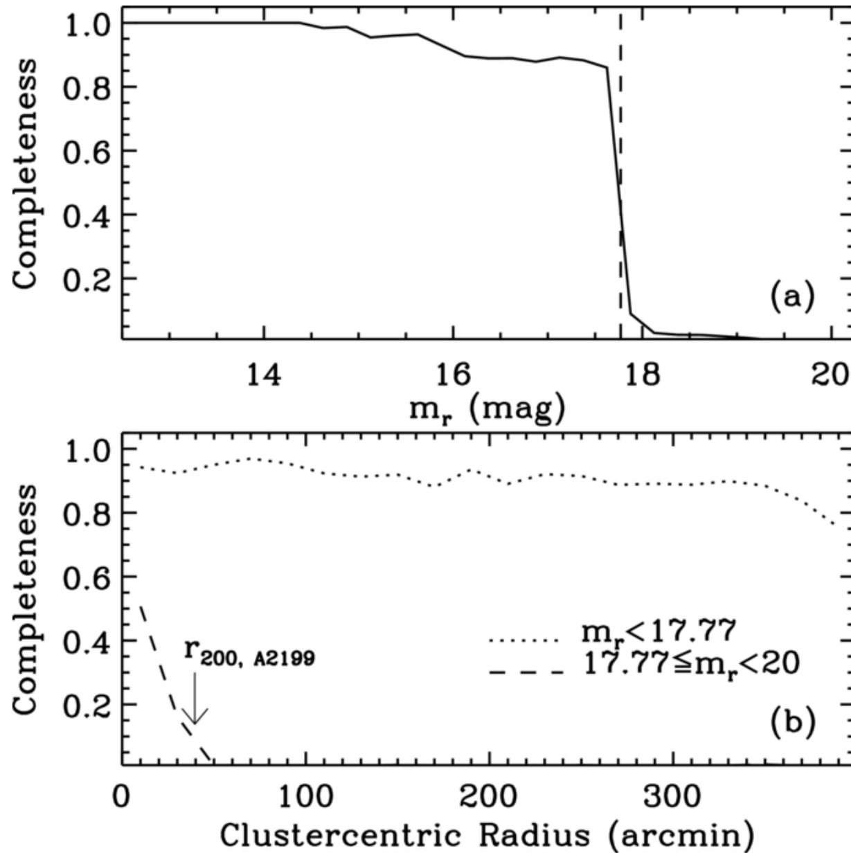
Figure 1. from A WISE View of a nearby Supercluster A2199 Hwang et al. 2012 ApJ 752 64 doi:10.1088/0004-637X/752/1/64 https://dx.doi.org/10.1088/0004-637X/752/1/64 © 2012. The American Astronomical Society. All rights reserved.
