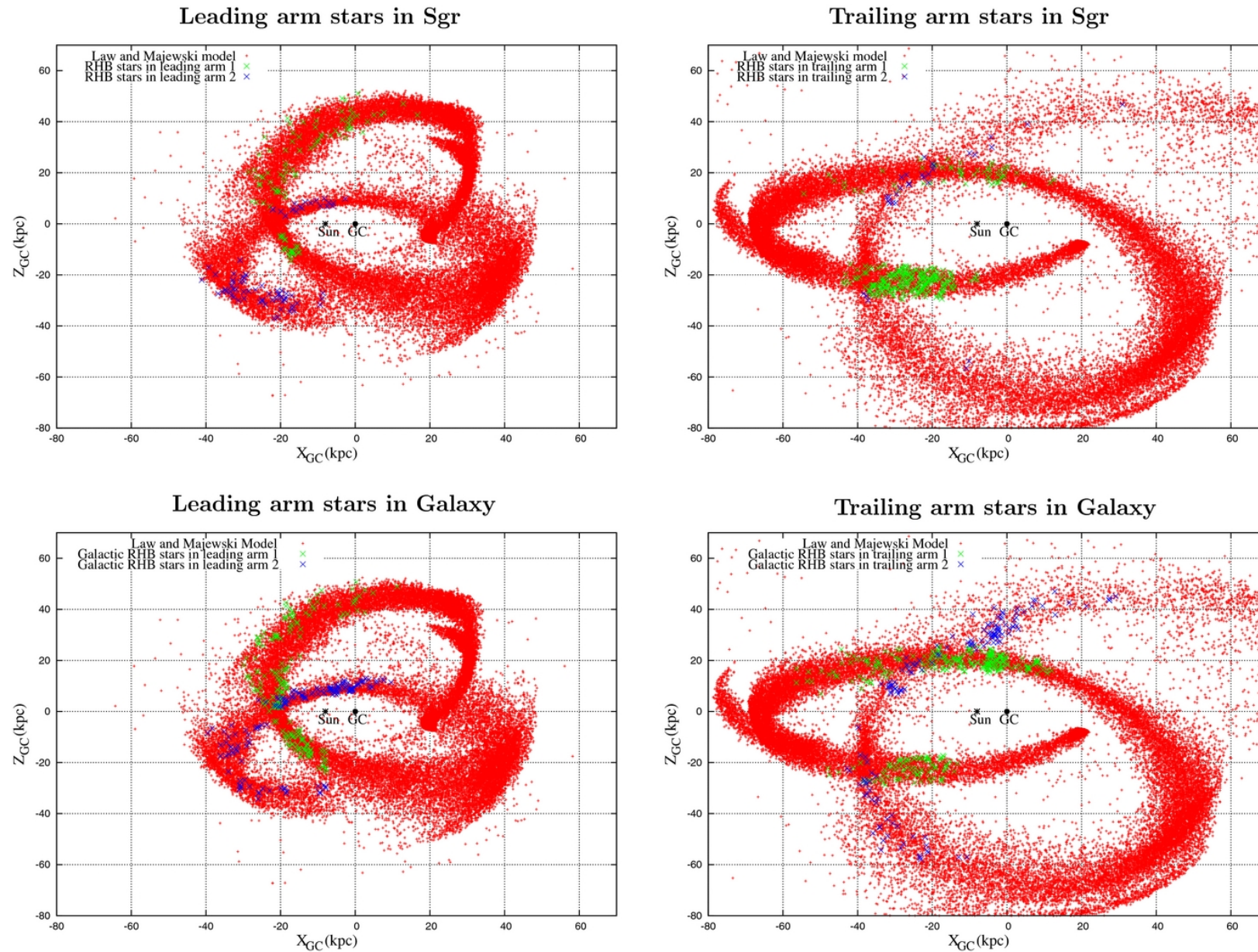
Figure 2. from The Kinematics and Chemistry of Red Horizontal Branch Stars in the Sagittarius Streams Shi et al. 2012 ApJ 751 130 doi:10.1088/0004-637X/751/2/130 https://dx.doi.org/10.1088/0004-637X/751/2/130 © 2012. The American Astronomical Society. All rights reserved.
