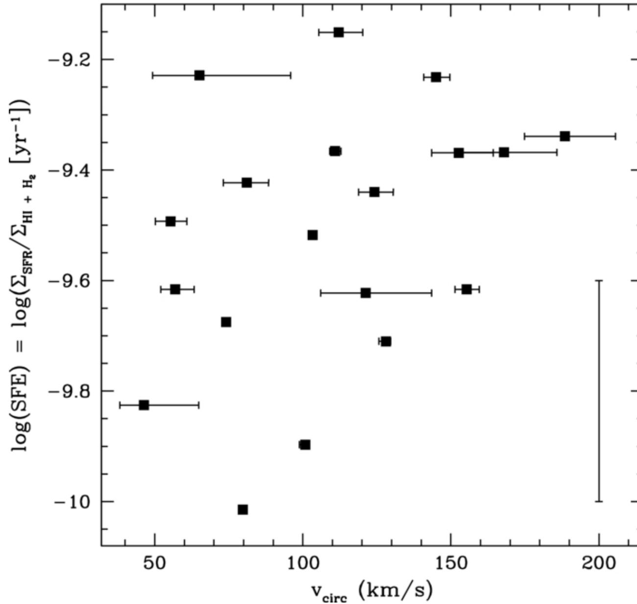
Figure 7. from Properties of Bulgeless Disk Galaxies. II. Star Formation as a Function of Circular Velocity Watson et al. 2012 ApJ 751 123 doi:10.1088/0004-637X/751/2/123 https://dx.doi.org/10.1088/0004-637X/751/2/123 © 2012. The American Astronomical Society. All rights reserved.
