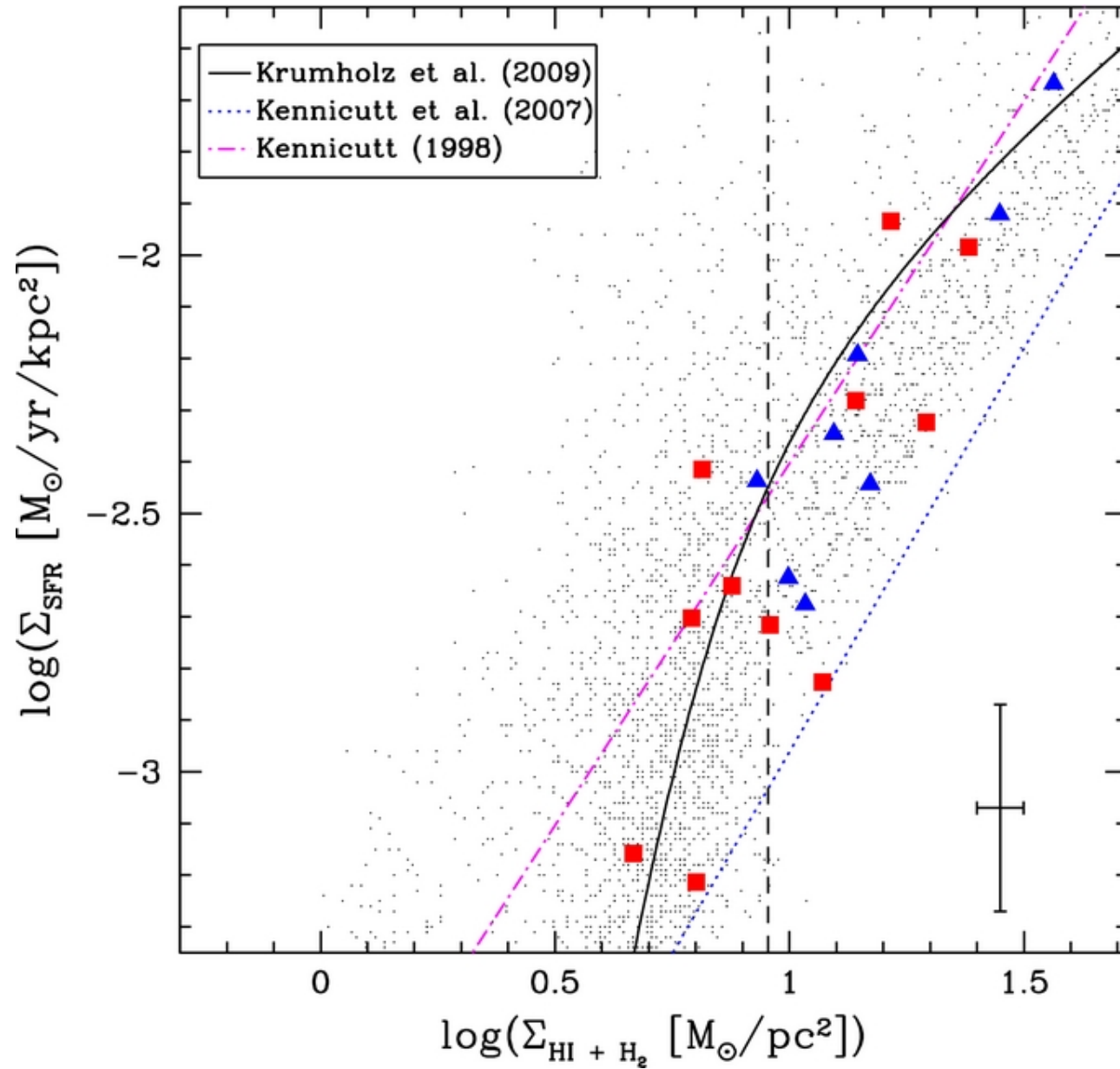
Figure 5. from Properties of Bulgeless Disk Galaxies. II. Star Formation as a Function of Circular Velocity Watson et al. 2012 ApJ 751 123 doi:10.1088/0004-637X/751/2/123 https://dx.doi.org/10.1088/0004-637X/751/2/123 © 2012. The American Astronomical Society. All rights reserved.
