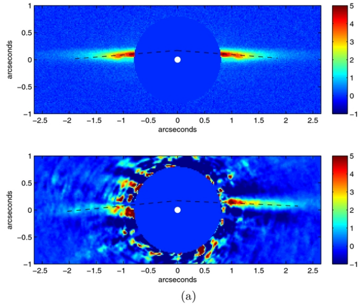
Figure 7. from The Gray Needle: Large Grains in the HD 15115 Debris Disk from LBT/PISCES/Ks and LBTI/LMIRcam/L Adaptive Optics Imaging Rodigas et al. 2012 ApJ 752 57 doi:10.1088/0004-637X/752/1/57 https://dx.doi.org/10.1088/0004-637X/752/1/57
