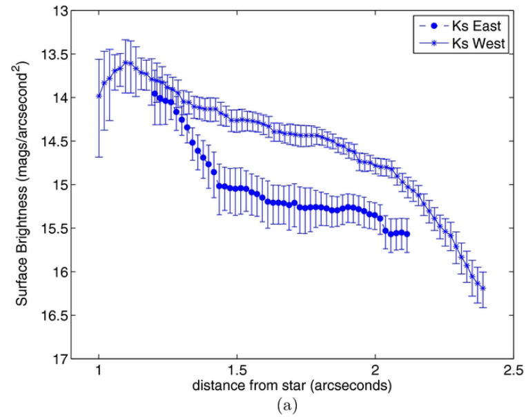
Figure 5. from The Gray Needle: Large Grains in the HD 15115 Debris Disk from LBT/PISCES/Ks and LBTI/LMIRcam/L Adaptive Optics Imaging Rodigas et al. 2012 ApJ 752 57 doi:10.1088/0004-637X/752/1/57 https://dx.doi.org/10.1088/0004-637X/752/1/57
