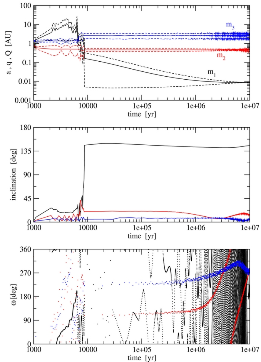
Figure 9. from Multiple-planet Scattering and the Origin of Hot Jupiters Beaugé & Nesvorný 2012 ApJ 751 119 doi:10.1088/0004-637X/751/2/119 https://dx.doi.org/10.1088/0004-637X/751/2/119 © 2012. The American Astronomical Society. All rights reserved.
