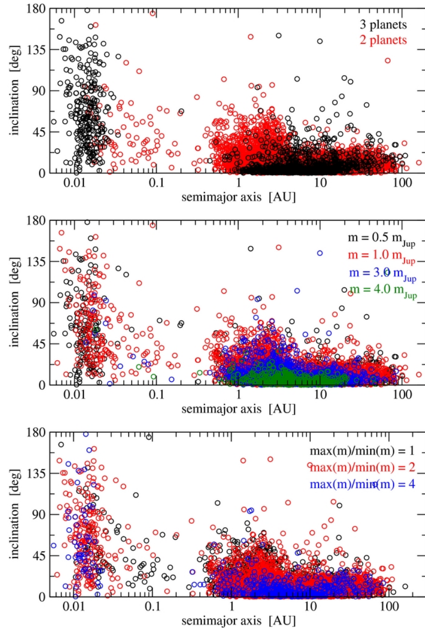
Figure 8. from Multiple-planet Scattering and the Origin of Hot Jupiters Beaugé & Nesvorný 2012 ApJ 751 119 doi:10.1088/0004-637X/751/2/119 https://dx.doi.org/10.1088/0004-637X/751/2/119
