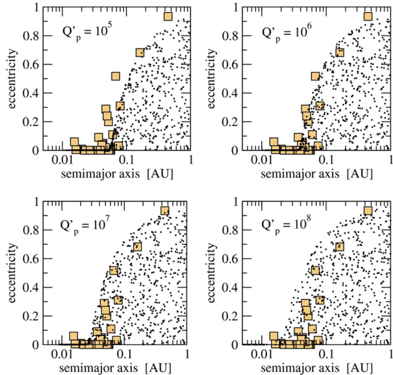
Figure 5. from Multiple-planet Scattering and the Origin of Hot Jupiters Beaugé & Nesvorný 2012 ApJ 751 119 doi:10.1088/0004-637X/751/2/119 https://dx.doi.org/10.1088/0004-637X/751/2/119 © 2012. The American Astronomical Society. All rights reserved.
