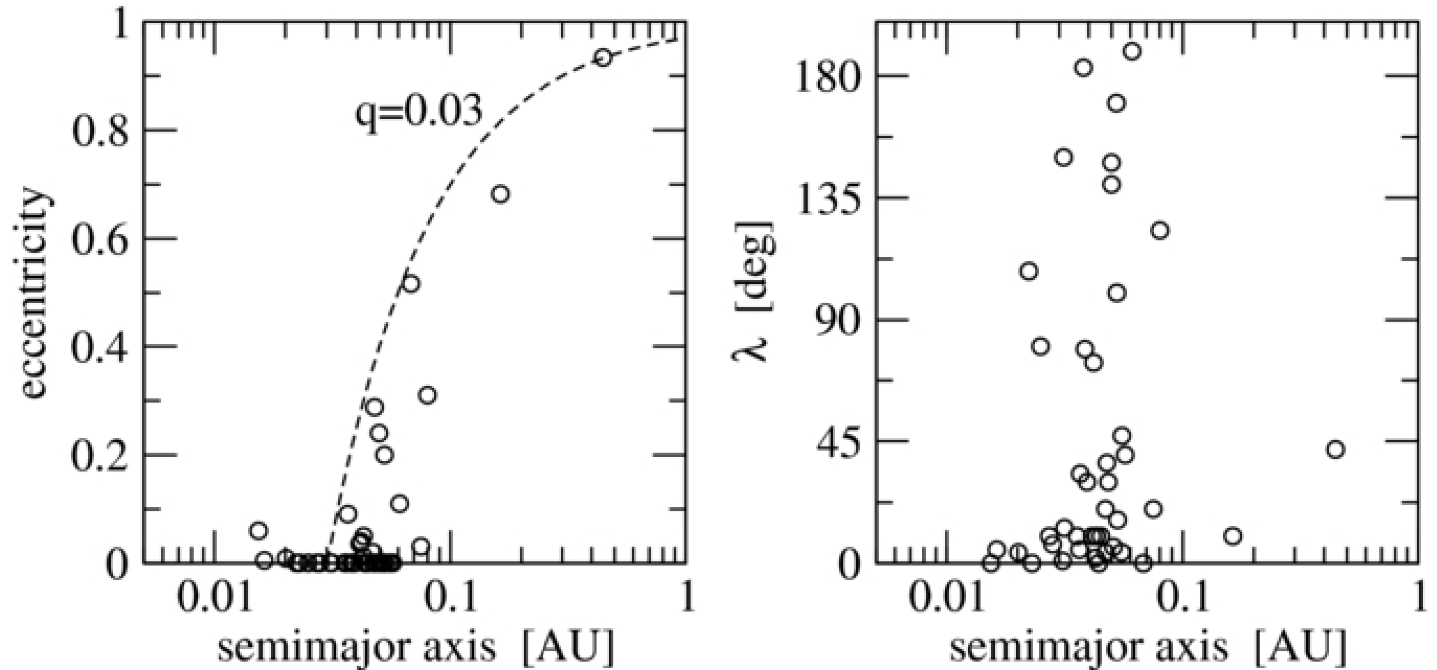
Figure 4. from Multiple-planet Scattering and the Origin of Hot Jupiters Beaugé & Nesvorný 2012 ApJ 751 119 doi:10.1088/0004-637X/751/2/119 https://dx.doi.org/10.1088/0004-637X/751/2/119 © 2012. The American Astronomical Society. All rights reserved.
