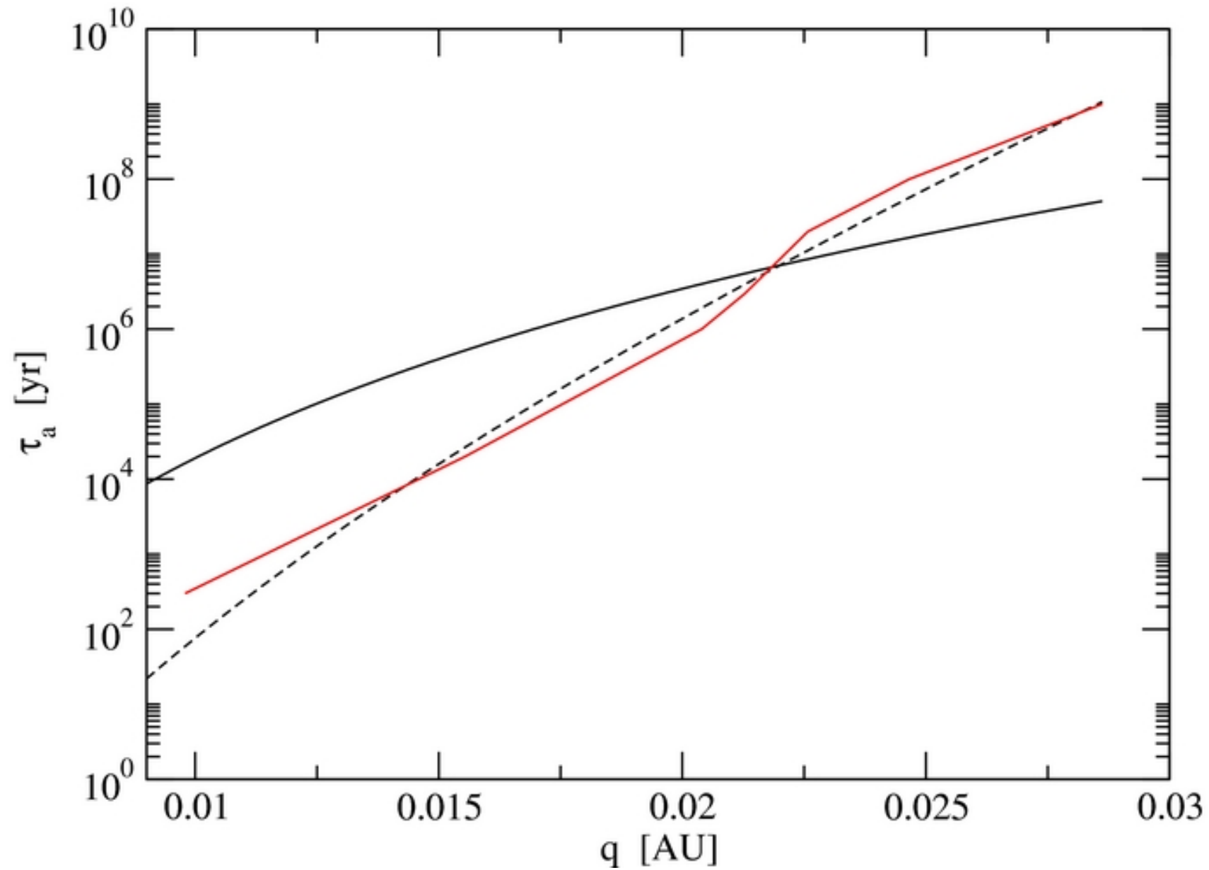
Figure 3. from Multiple-planet Scattering and the Origin of Hot Jupiters Beaugé & Nesvorný 2012 ApJ 751 119 doi:10.1088/0004-637X/751/2/119 https://dx.doi.org/10.1088/0004-637X/751/2/119 © 2012. The American Astronomical Society. All rights reserved.
