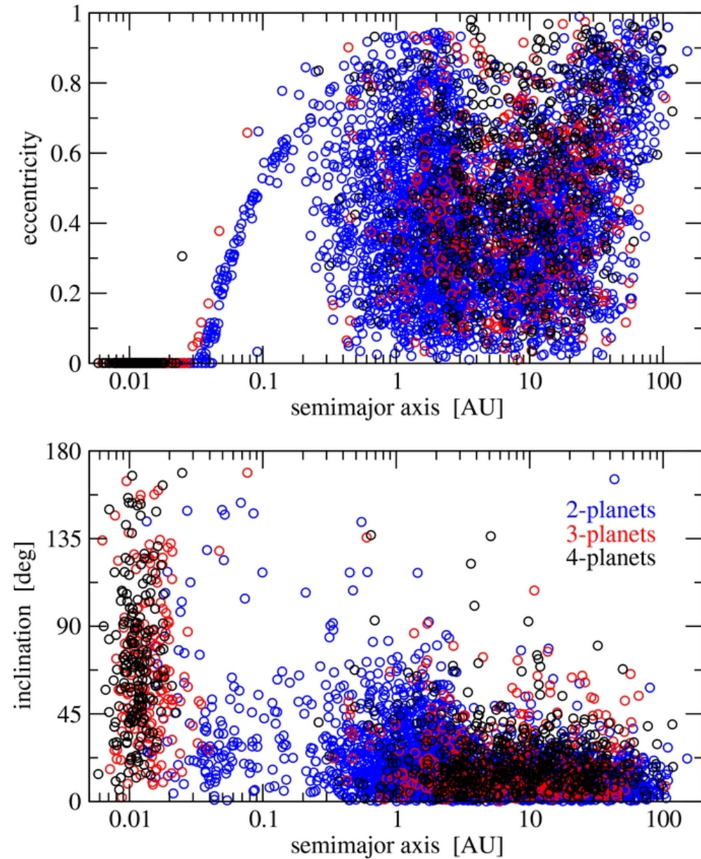
Figure 13. from Multiple-planet Scattering and the Origin of Hot Jupiters Beaugé & Nesvorný 2012 ApJ 751 119 doi:10.1088/0004-637X/751/2/119 https://dx.doi.org/10.1088/0004-637X/751/2/119 © 2012. The American Astronomical Society. All rights reserved.
