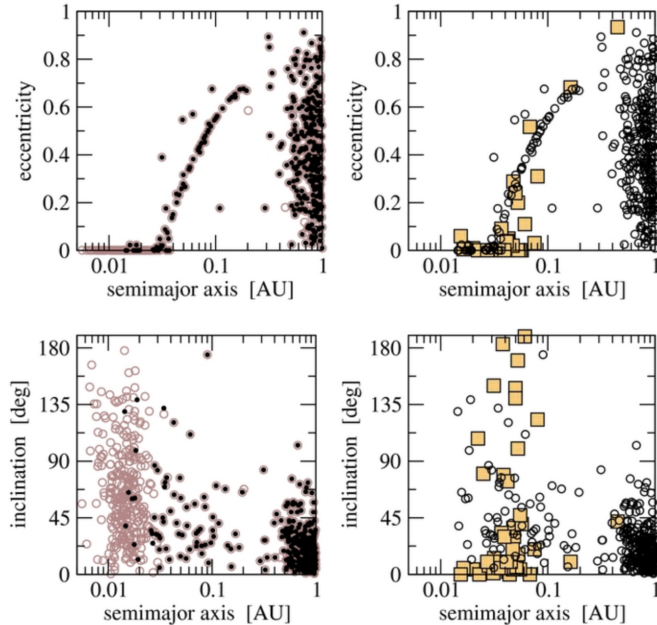
Figure 12. from Multiple-planet Scattering and the Origin of Hot Jupiters Beaugé & Nesvorný 2012 ApJ 751 119 doi:10.1088/0004-637X/751/2/119 https://dx.doi.org/10.1088/0004-637X/751/2/119 © 2012. The American Astronomical Society. All rights reserved.
