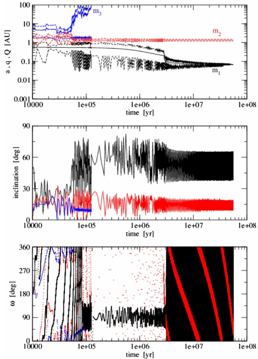
Figure 11. from Multiple-planet Scattering and the Origin of Hot Jupiters Beaugé & Nesvorný 2012 ApJ 751 119 doi:10.1088/0004-637X/751/2/119 https://dx.doi.org/10.1088/0004-637X/751/2/119
