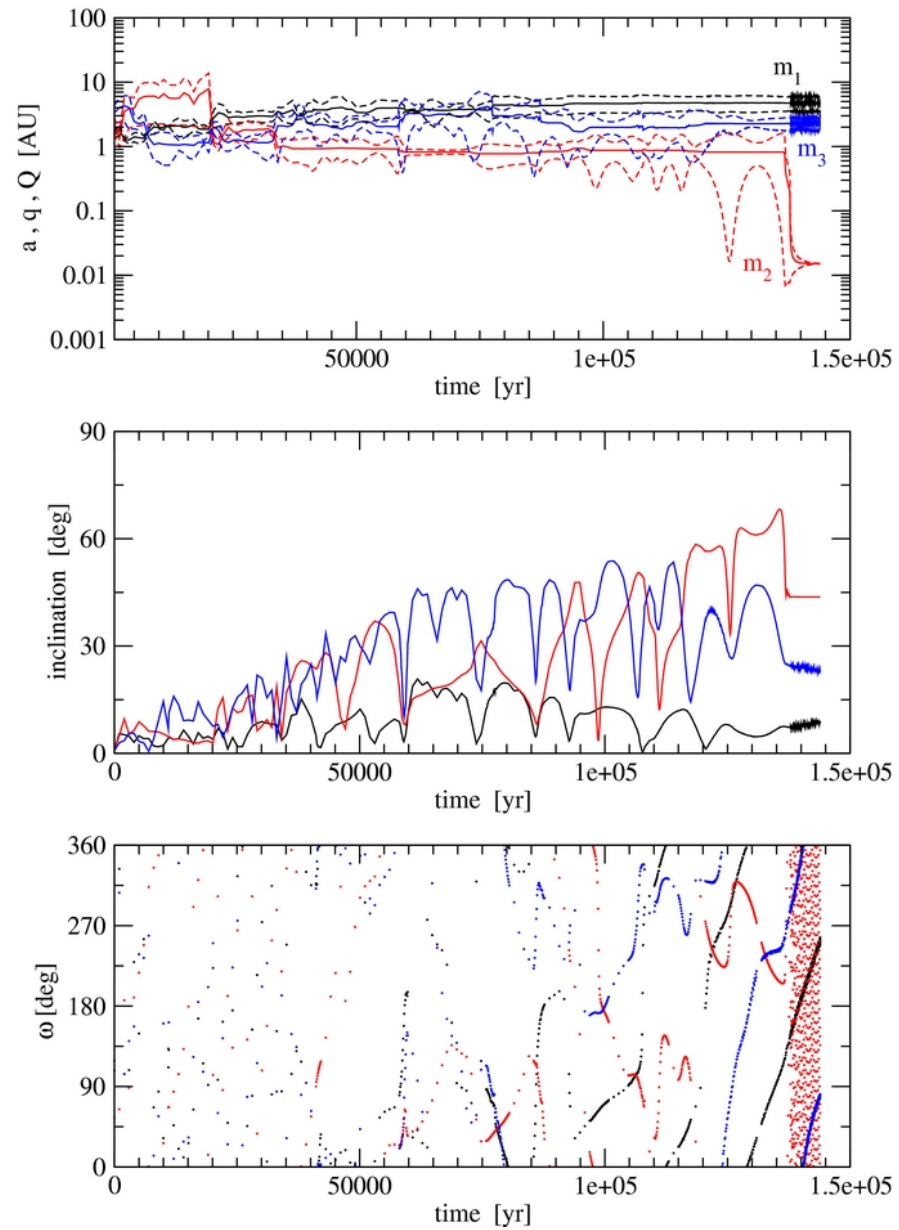
Figure 10. from Multiple-planet Scattering and the Origin of Hot Jupiters Beaugé & Nesvorný 2012 ApJ 751 119 doi:10.1088/0004-637X/751/2/119 https://dx.doi.org/10.1088/0004-637X/751/2/119 © 2012. The American Astronomical Society. All rights reserved.
