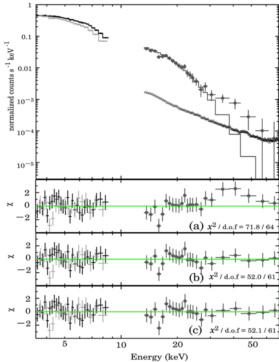
Figure 8. from Possible Detection of an Emission Cyclotron Resonance Scattering Feature from the Accretion-powered Pulsar 4U 1626–67 Iwakiri et al. 2012 ApJ 751 35 doi:10.1088/0004-637X/751/1/35 https://dx.doi.org/10.1088/0004-637X/751/1/35 © 2012. The American Astronomical Society. All rights reserved.
