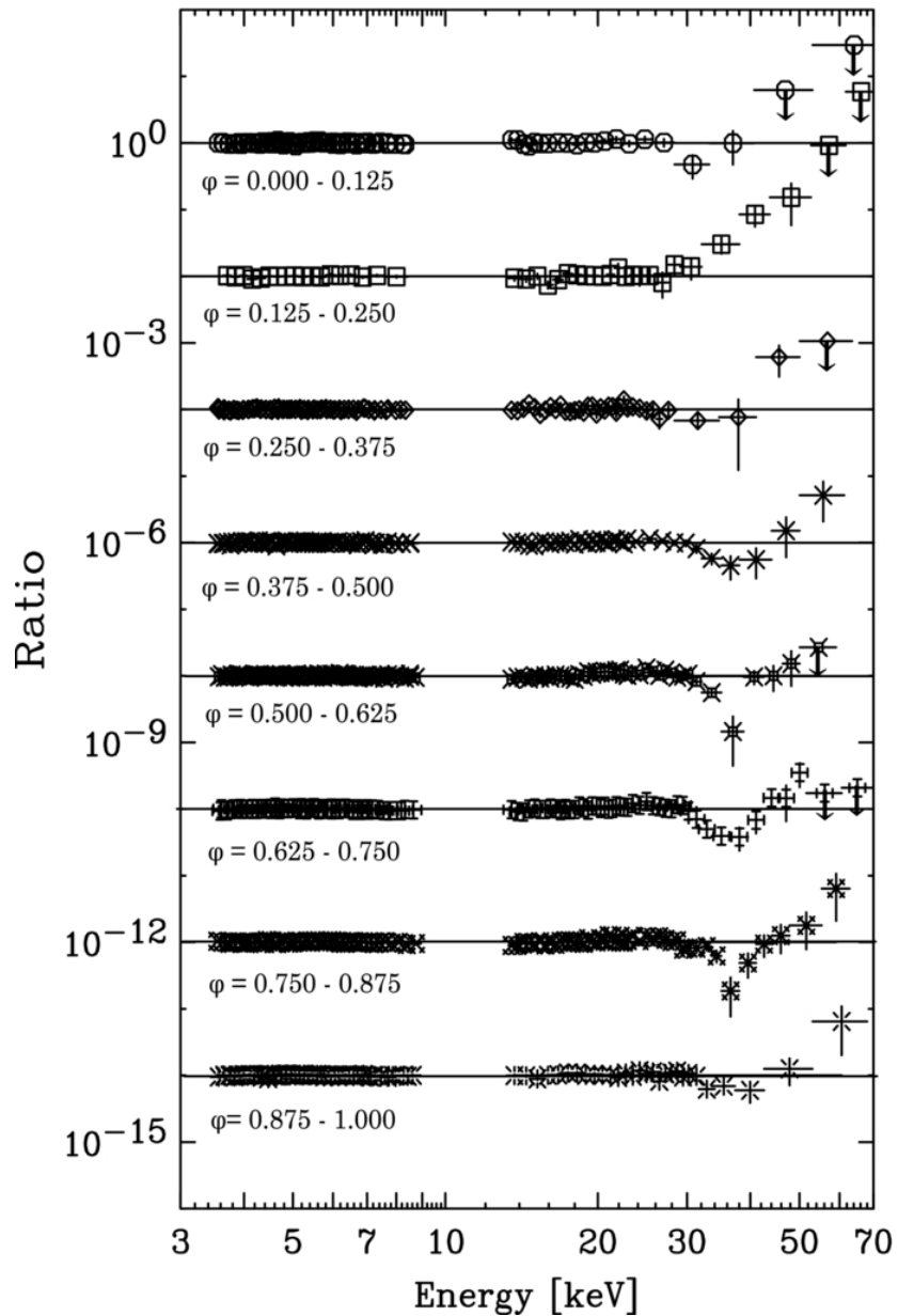
Figure 7. from Possible Detection of an Emission Cyclotron Resonance Scattering Feature from the Accretion-powered Pulsar 4U 1626–67 Iwakiri et al. 2012 ApJ 751 35 doi:10.1088/0004-637X/751/1/35 https://dx.doi.org/10.1088/0004-637X/751/1/35 © 2012. The American Astronomical Society. All rights reserved.
