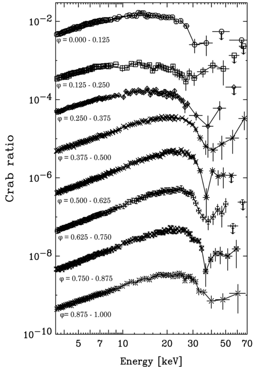
Figure 6. from Possible Detection of an Emission Cyclotron Resonance Scattering Feature from the Accretion-powered Pulsar 4U 1626–67 Iwakiri et al. 2012 ApJ 751 35 doi:10.1088/0004-637X/751/1/35 https://dx.doi.org/10.1088/0004-637X/751/1/35 © 2012. The American Astronomical Society. All rights reserved.
