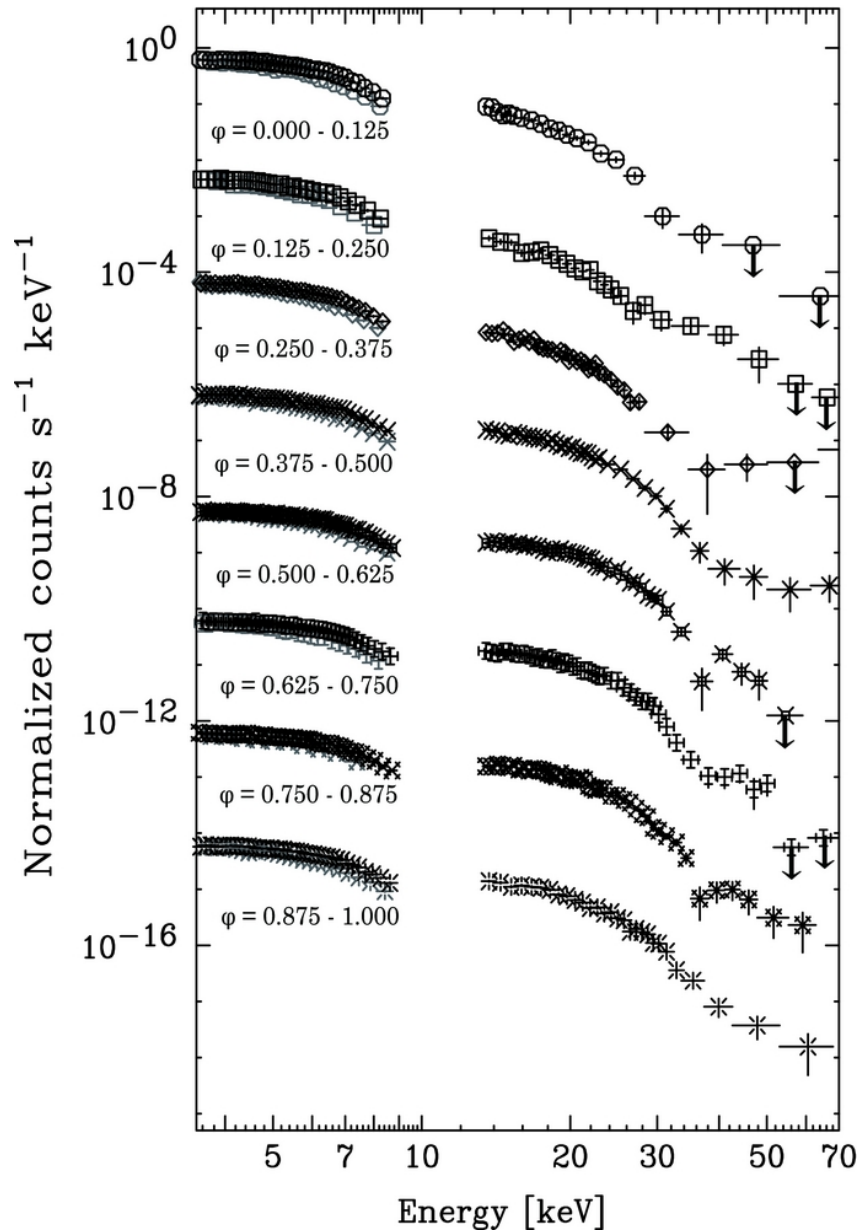
Figure 5. from Possible Detection of an Emission Cyclotron Resonance Scattering Feature from the Accretion-powered Pulsar 4U 1626–67 Iwakiri et al. 2012 ApJ 751 35 doi:10.1088/0004-637X/751/1/35 https://dx.doi.org/10.1088/0004-637X/751/1/35 © 2012. The American Astronomical Society. All rights reserved.
