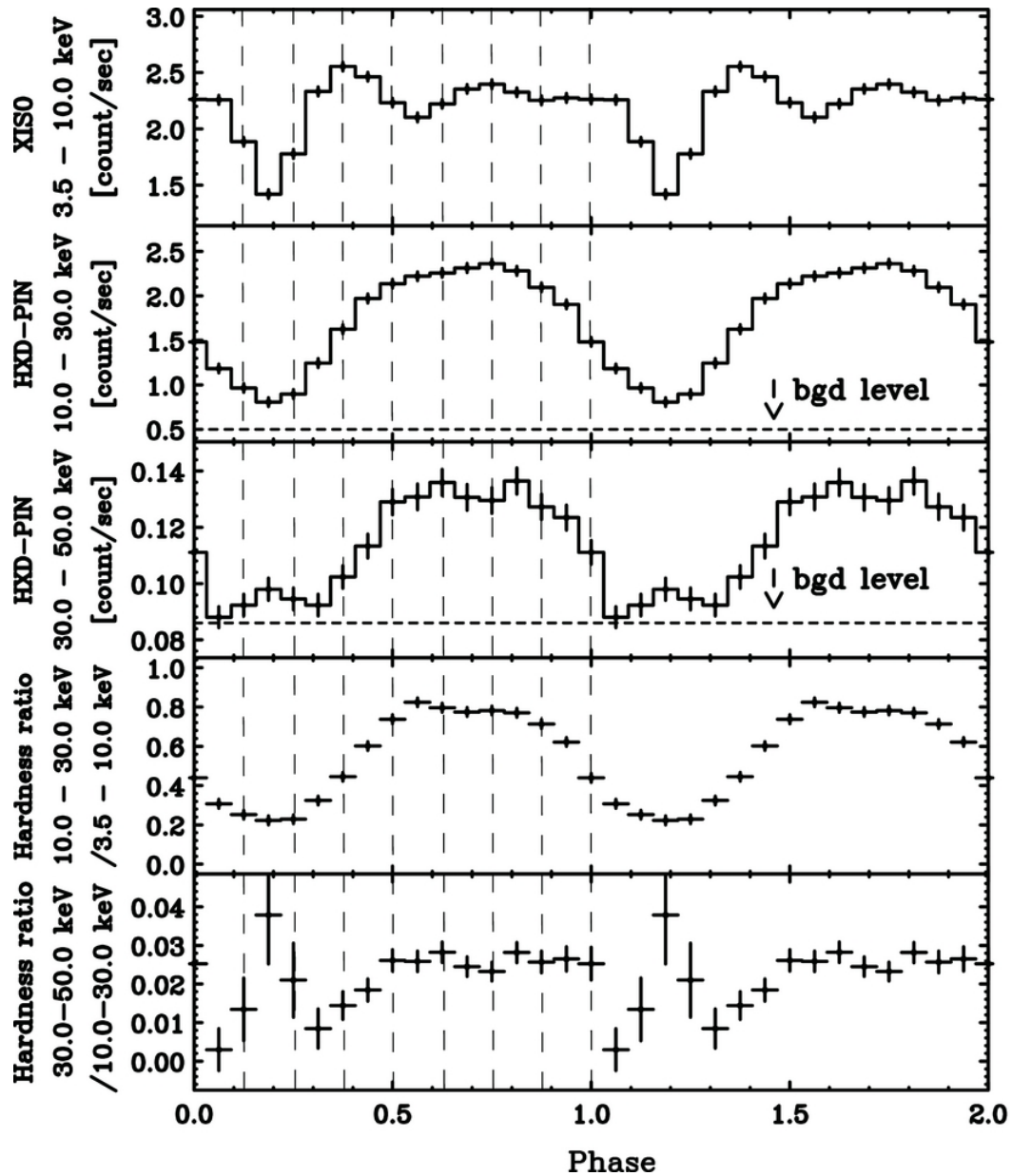
Figure 4. from Possible Detection of an Emission Cyclotron Resonance Scattering Feature from the Accretion-powered Pulsar 4U 1626–67 Iwakiri et al. 2012 ApJ 751 35 doi:10.1088/0004-637X/751/1/35 https://dx.doi.org/10.1088/0004-637X/751/1/35
