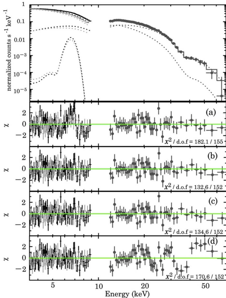
Figure 3. from Possible Detection of an Emission Cyclotron Resonance Scattering Feature from the Accretion-powered Pulsar 4U 1626–67 Iwakiri et al. 2012 ApJ 751 35 doi:10.1088/0004-637X/751/1/35 https://dx.doi.org/10.1088/0004-637X/751/1/35 © 2012. The American Astronomical Society. All rights reserved.
